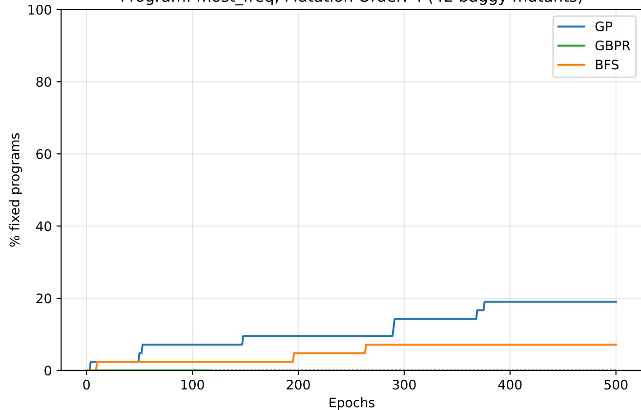
Program: most_freq, Mutation Order: 4 (42 buggy mutants)
