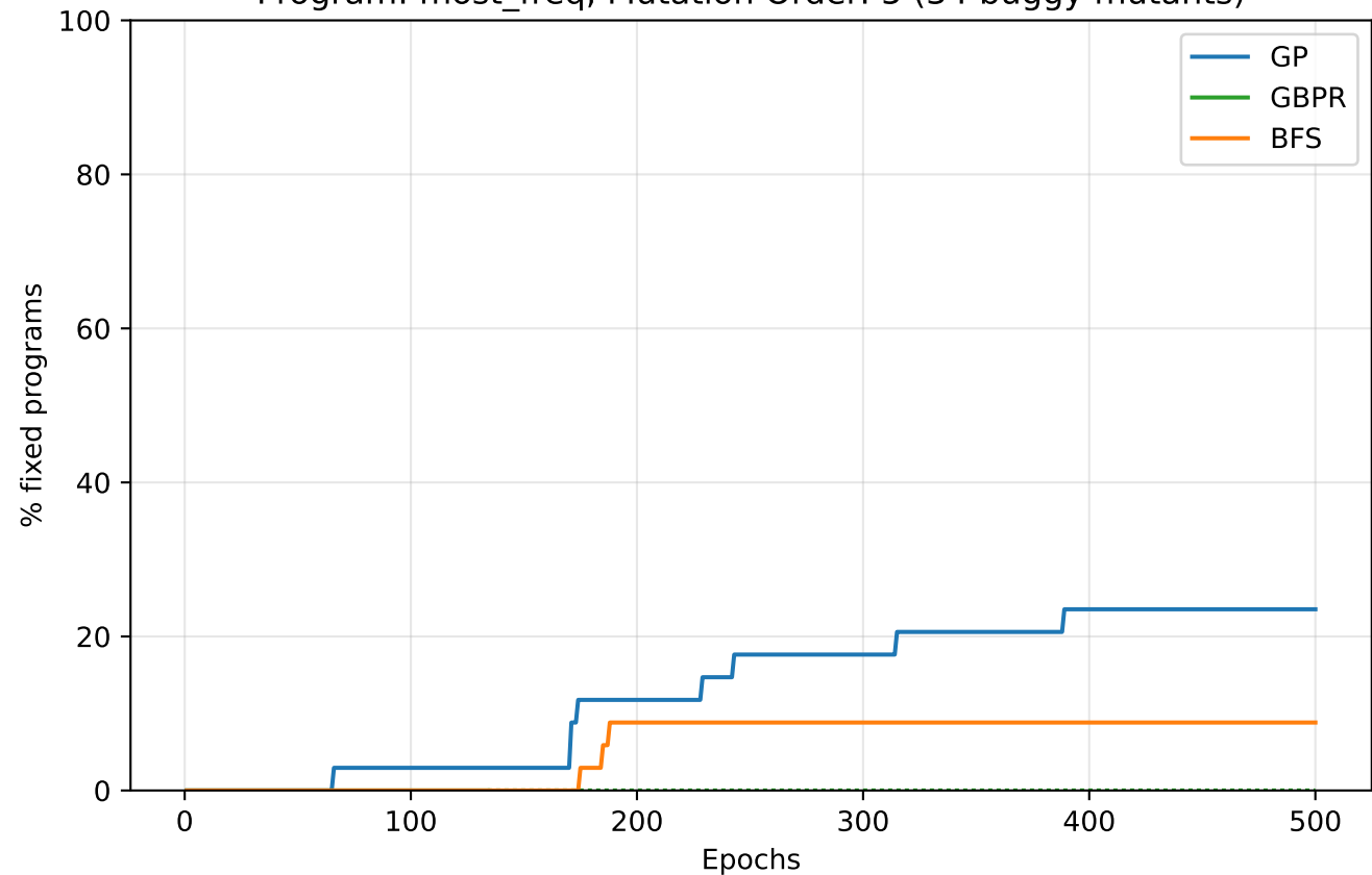
Program: most_freq, Mutation Order: 5 (34 buggy mutants)
