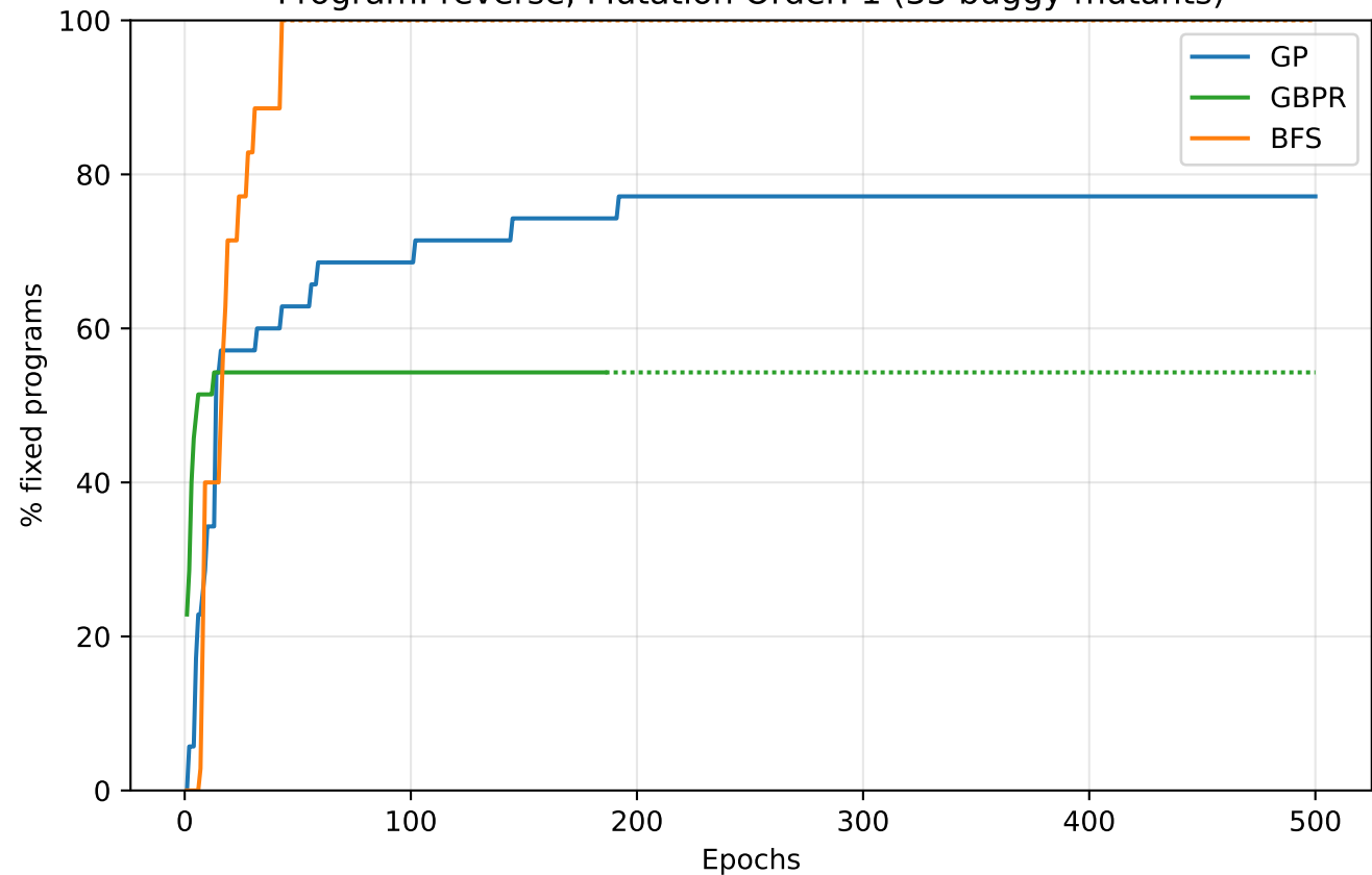
Program: reverse, Mutation Order: 1 (35 buggy mutants)
