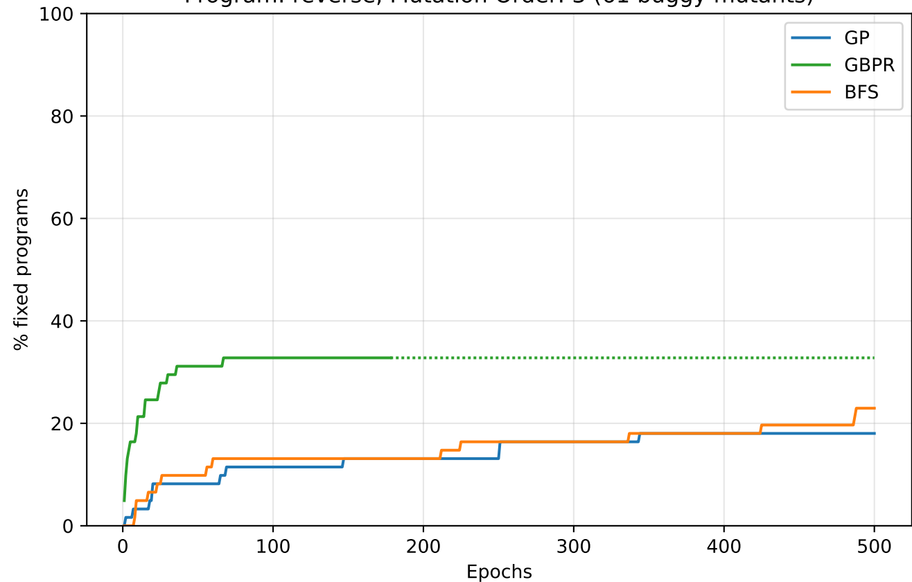
Program: reverse, Mutation Order: 3 (61 buggy mutants)
