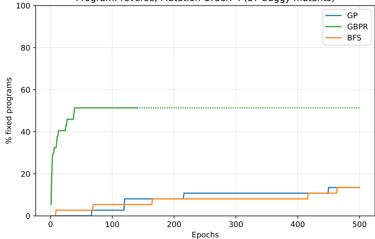
Program: reverse, Mutation Order: 4 (37 buggy mutants)
