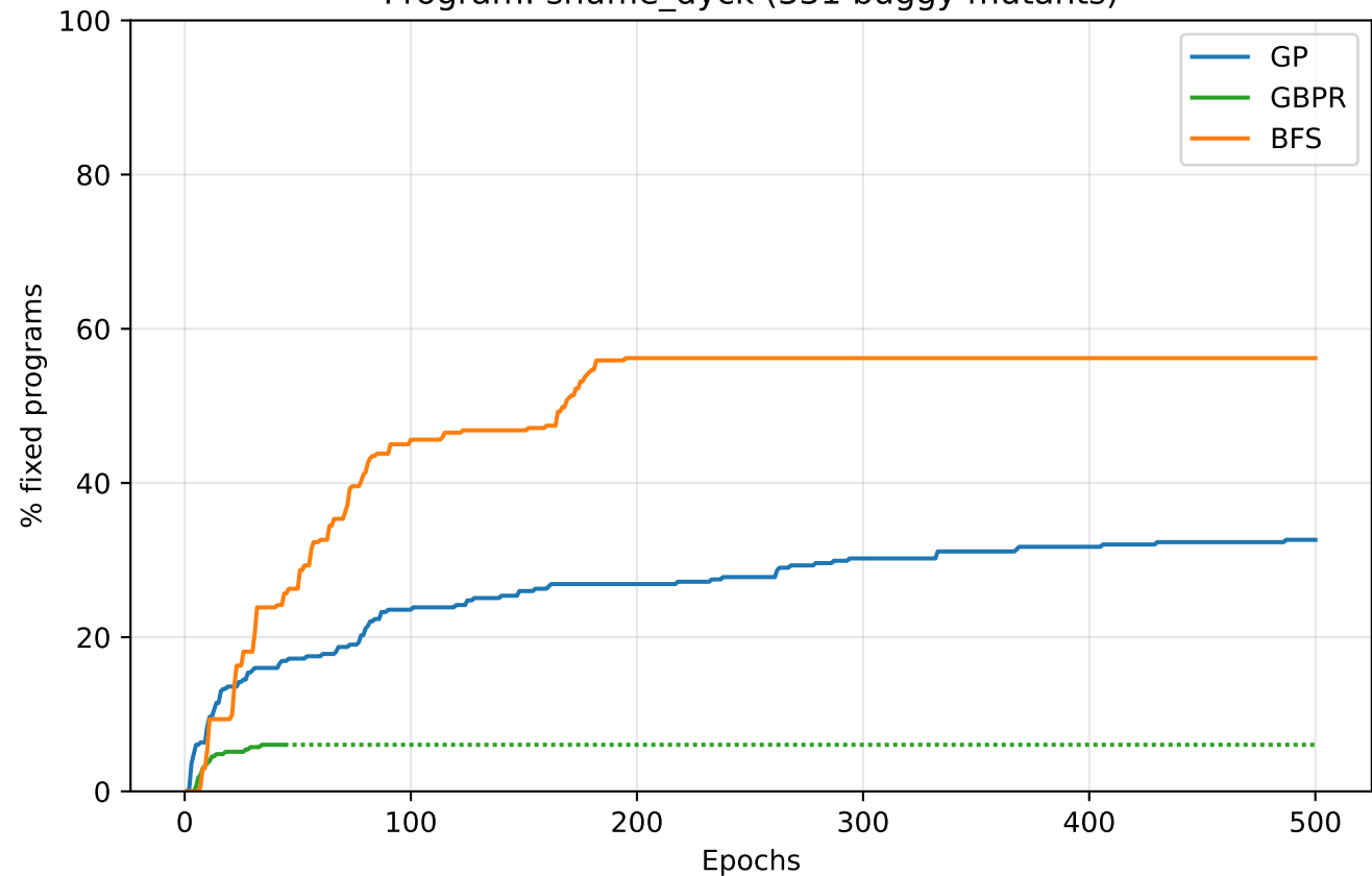
Program: shuffle_dyck (331 buggy mutants)
