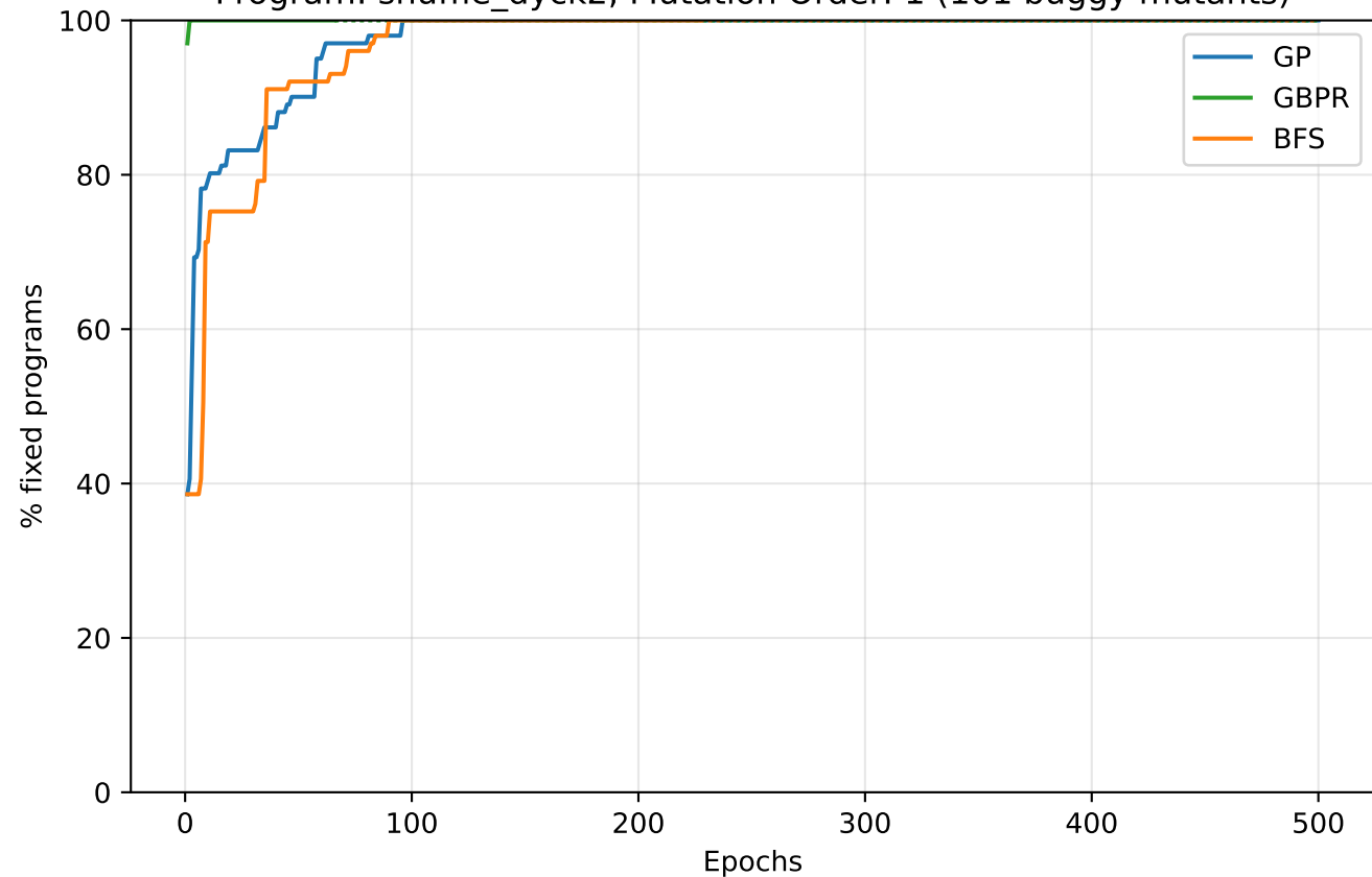
Program: shuffle_dyck2, Mutation Order: 1 (101 buggy mutants)
