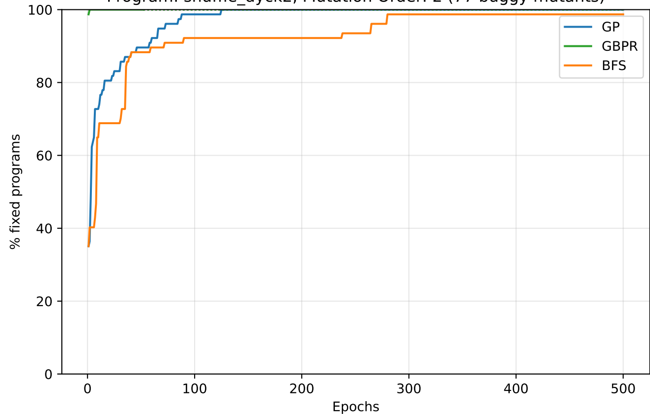
Program: shuffle_dyck2, Mutation Order: 2 (77 buggy mutants)
