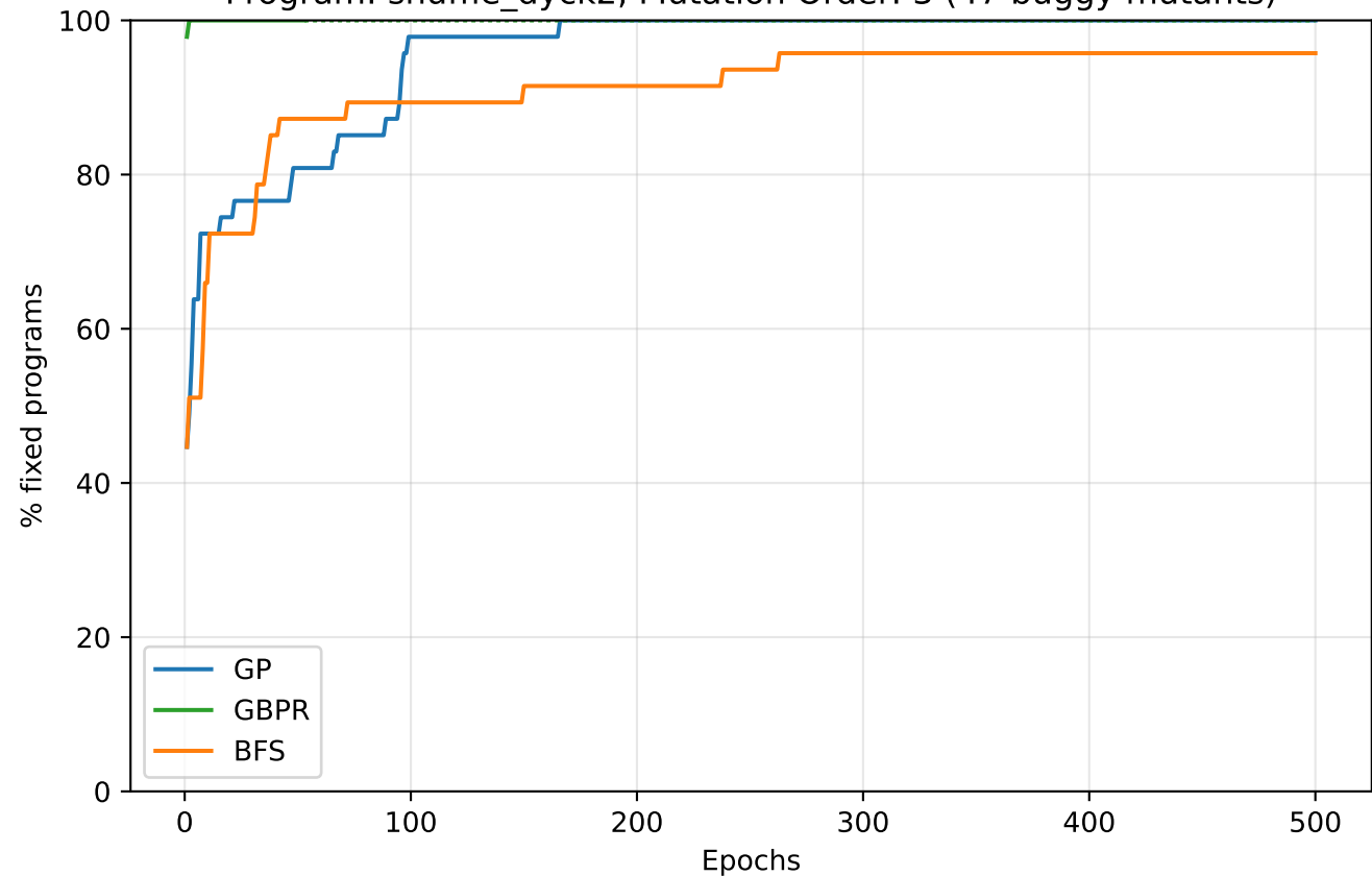
Program: shuffle_dyck2, Mutation Order: 3 (47 buggy mutants)
