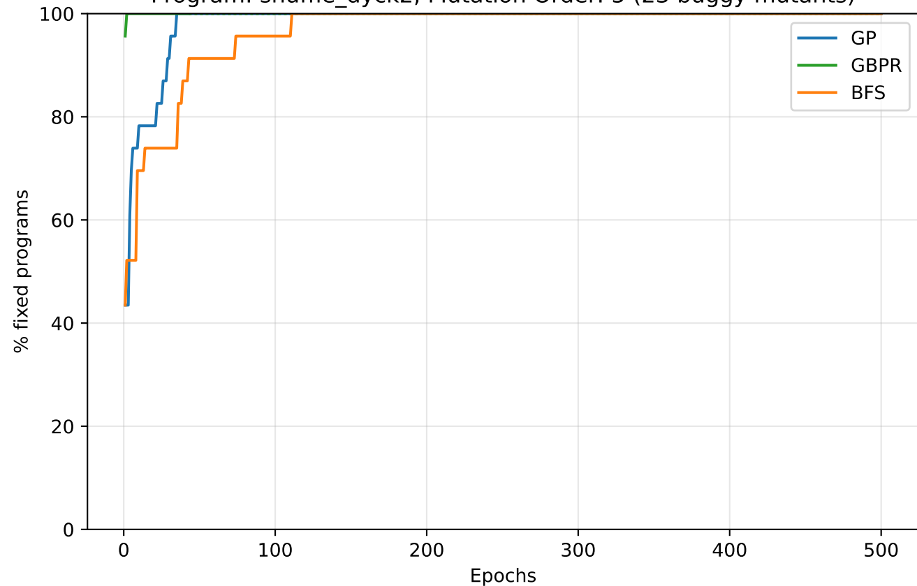
Program: shuffle_dyck2, Mutation Order: 5 (23 buggy mutants)
