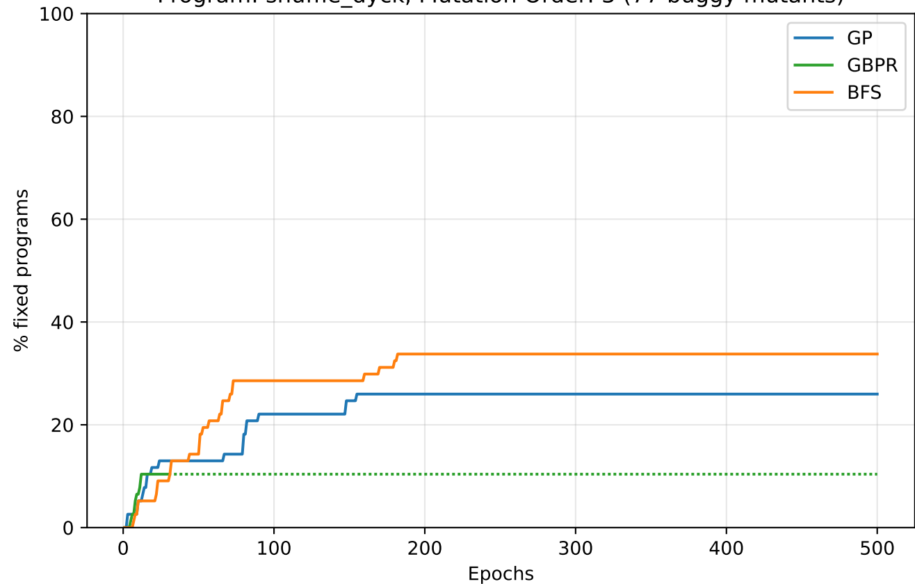
Program: shuffle_dyck, Mutation Order: 3 (77 buggy mutants)
