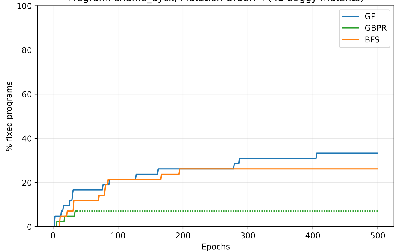
Program: shuffle_dyck, Mutation Order: 4 (42 buggy mutants)
