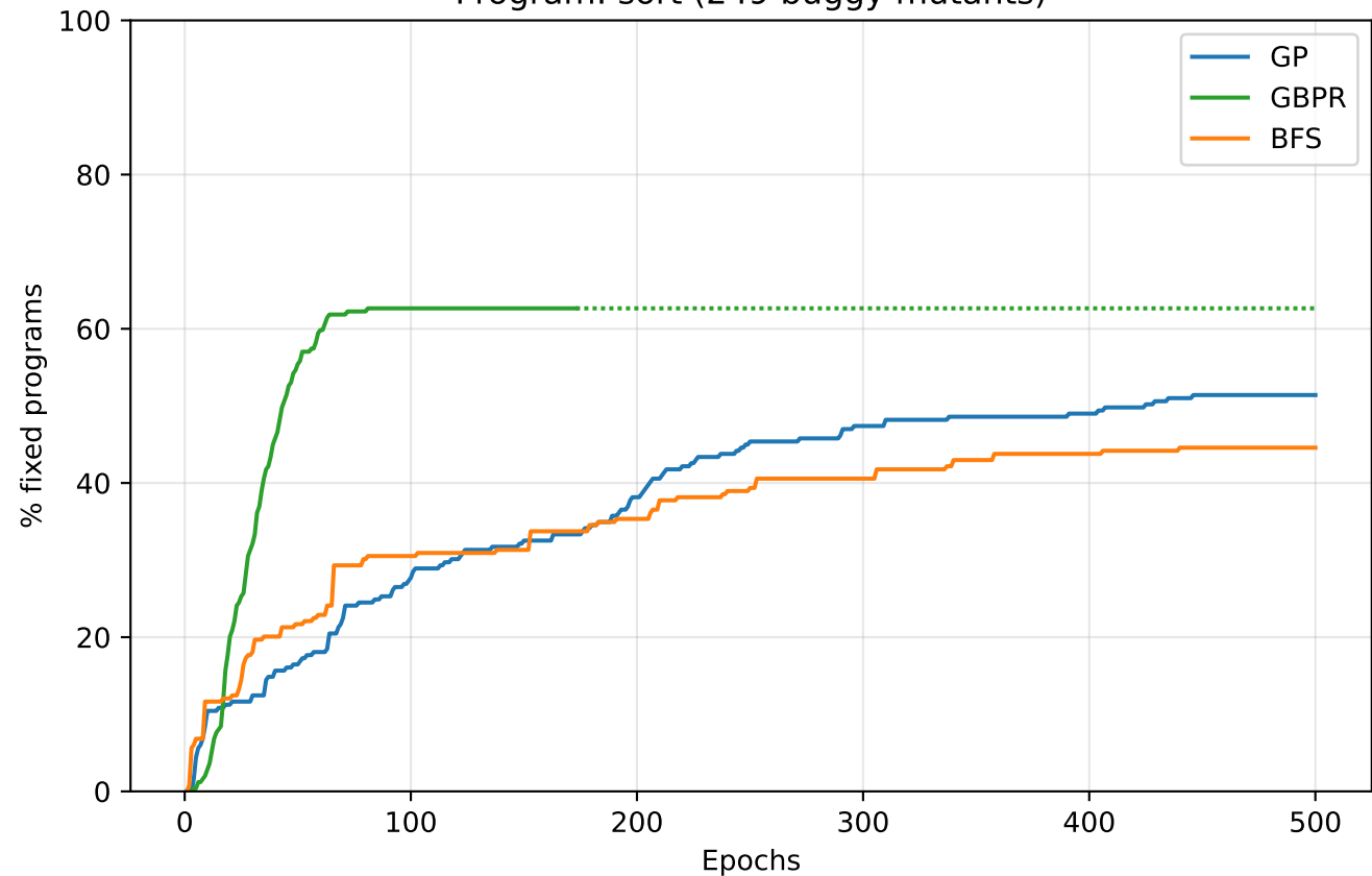
Program: sort (249 buggy mutants)
