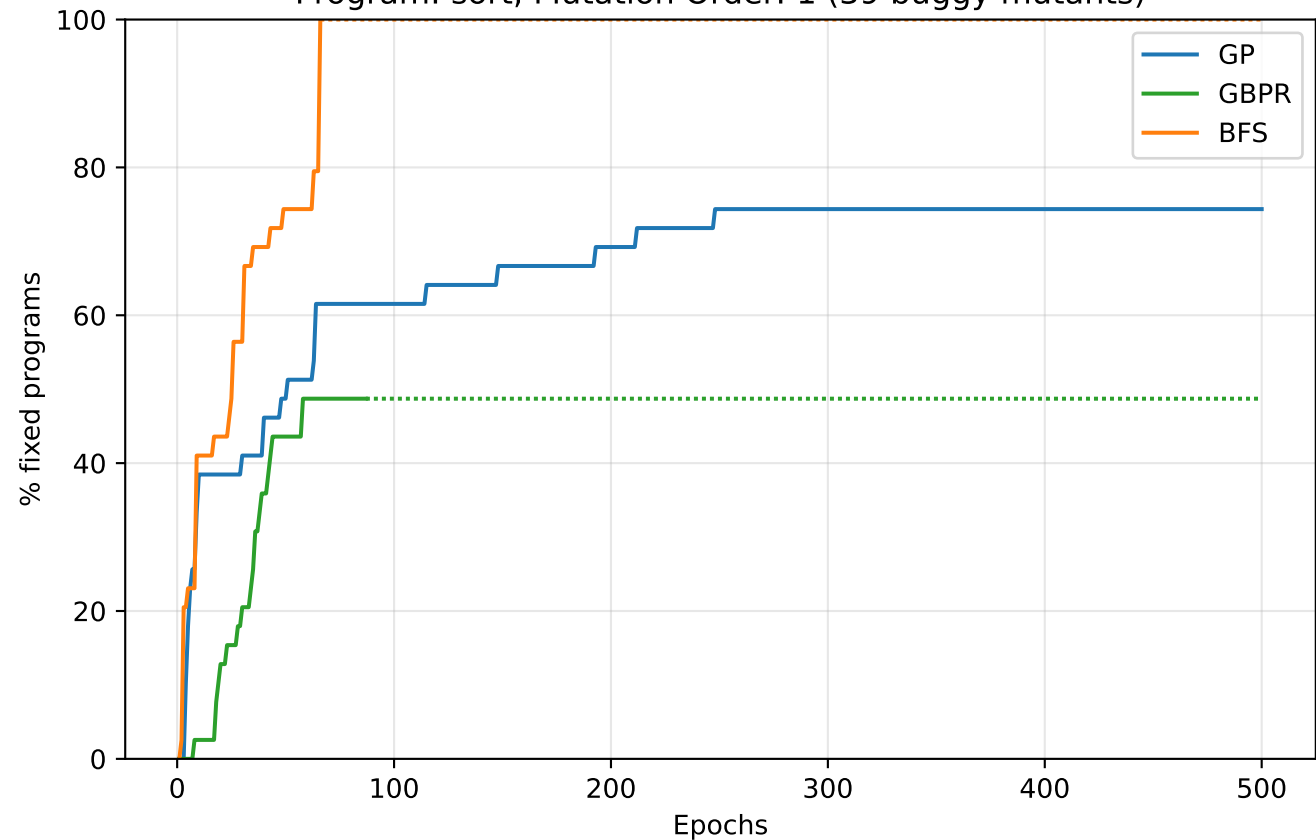
Program: sort, Mutation Order: 1 (39 buggy mutants)
