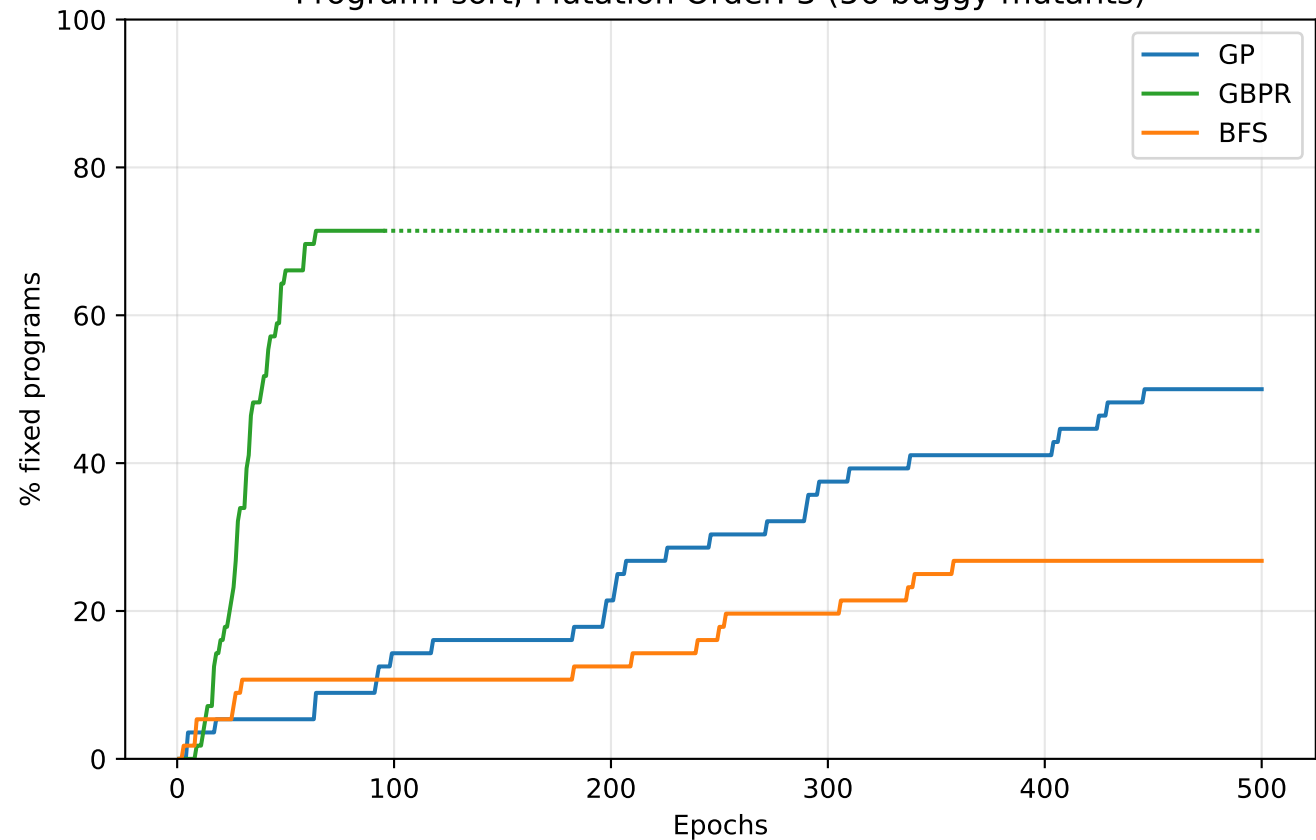
Program: sort, Mutation Order: 3 (56 buggy mutants)
