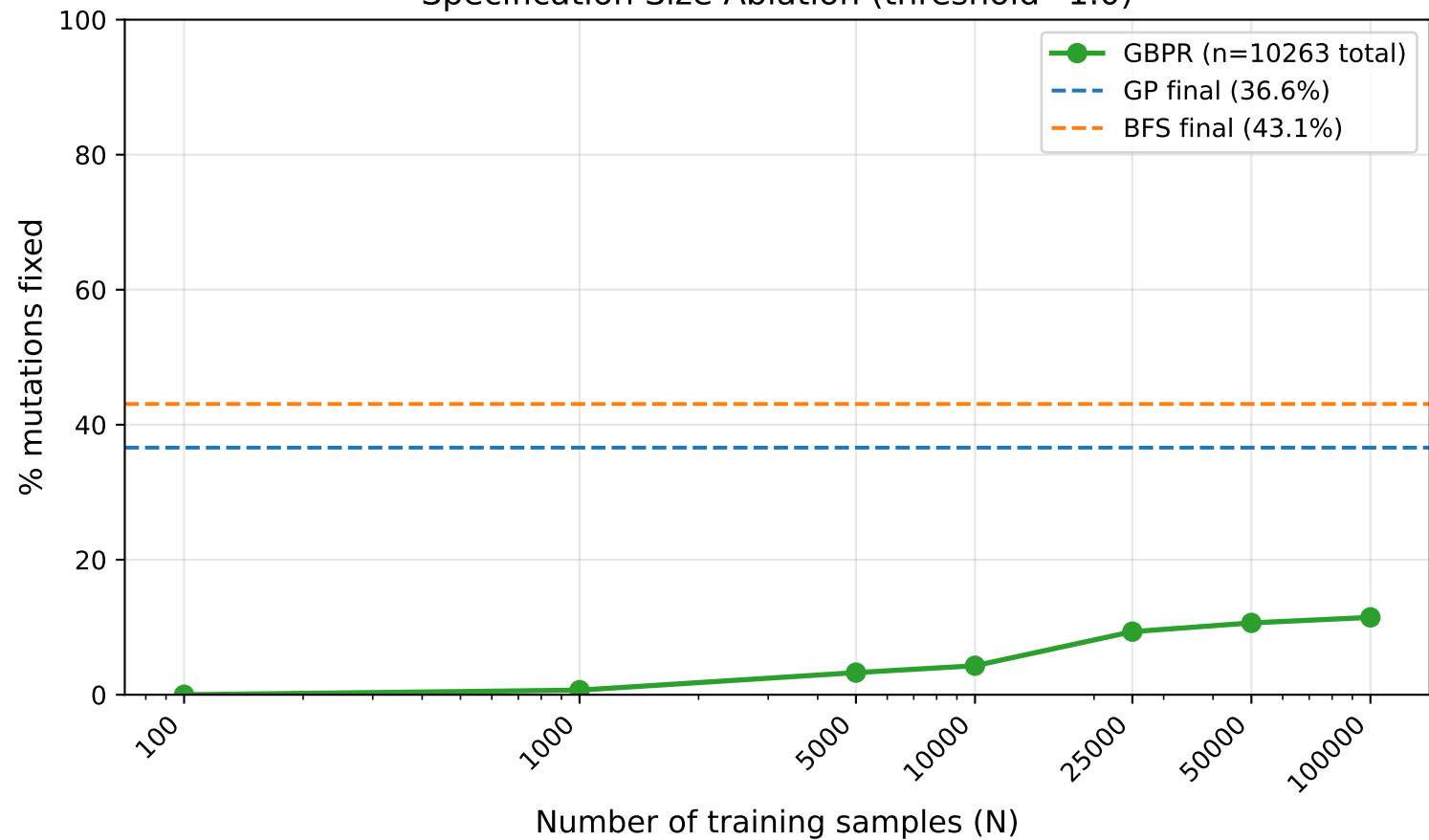
Specification Size Ablation (threshold=1.0)
