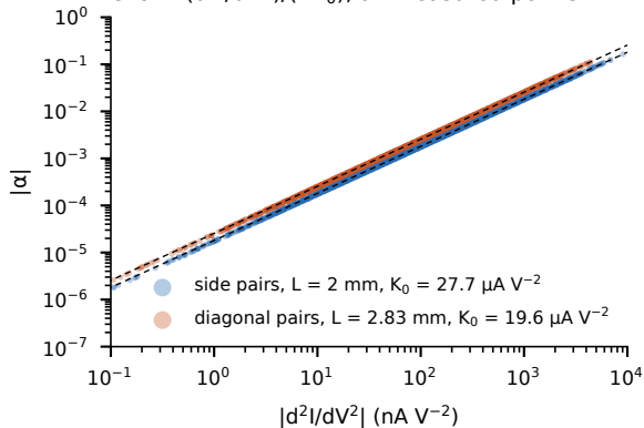
c \alpha = (d^2I/dV^2)/(2K_0) , all measured points
