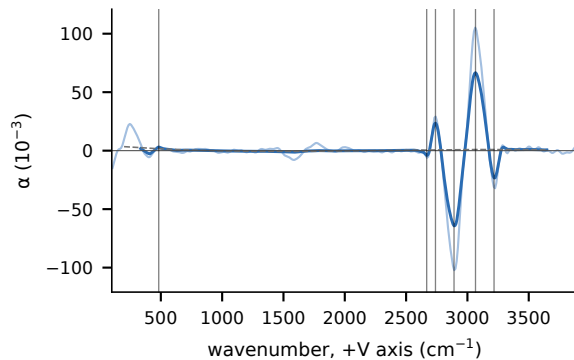
b impure device, pair 23_32 ( L = 2.8 mm)
