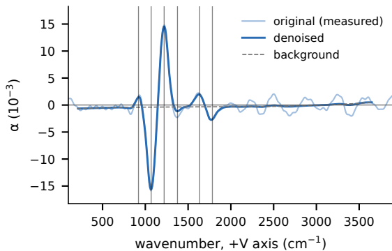
a pure device, pair 22_31 ( L = 2.8 mm)
