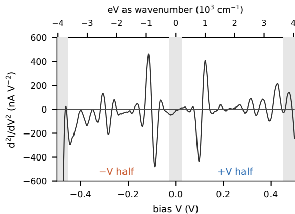
a one full sweep (pure device, pair 41_52)
