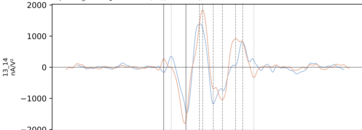
impure 13_14 — aligned: -V \approx \pm(+V)(1.12 \cdot w - 312) , r=0.86
