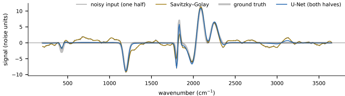
a held-out simulated spectrum
