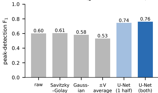
b simulated test set (ground truth known)
