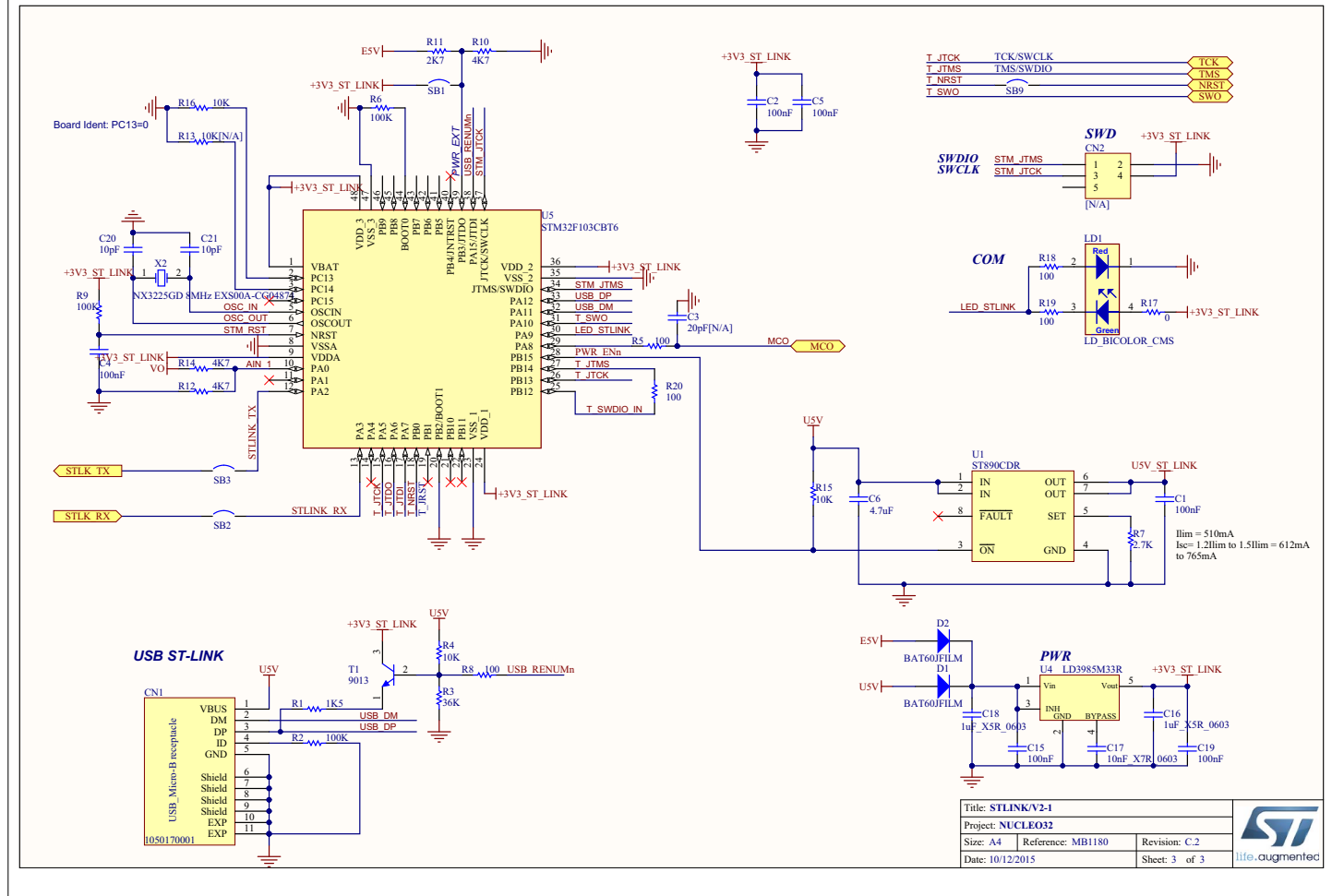
Figure 11. ST-LINK/V2-1
