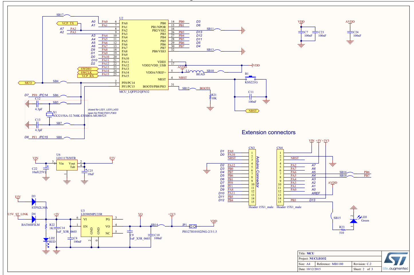
Figure 10. MCU
