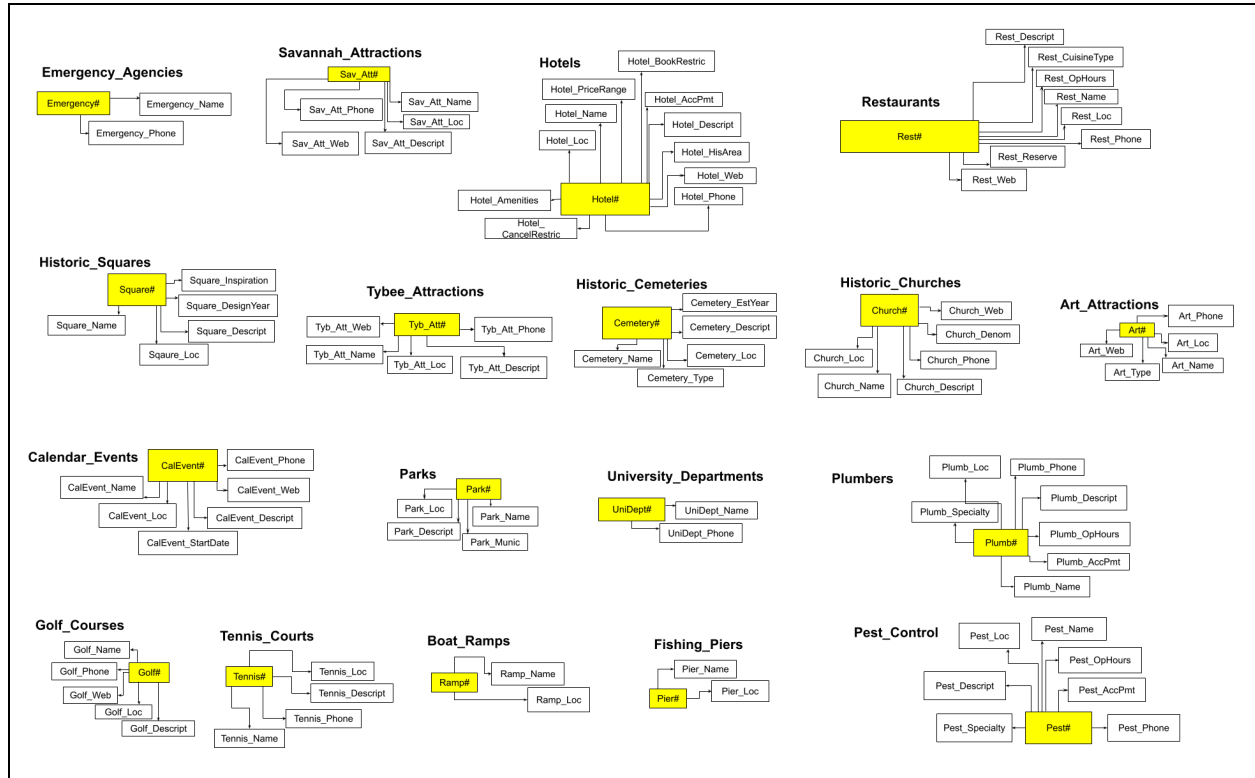
Figure 8: Diagram of remaining relations in 4NF
