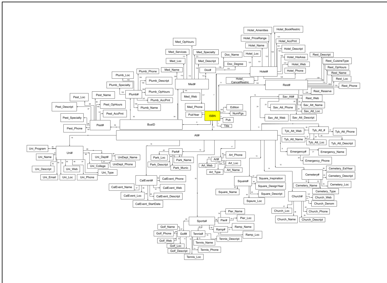
Figure 1: Initial FD Diagram
