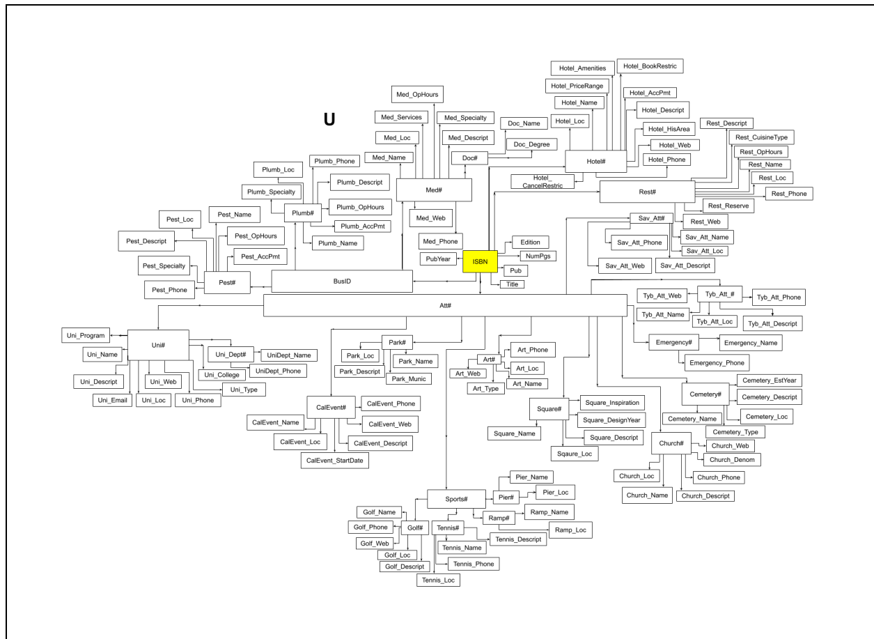
Figure 3: Diagram of the relation in 1NF (same as Figure 1 & Figure 2)
