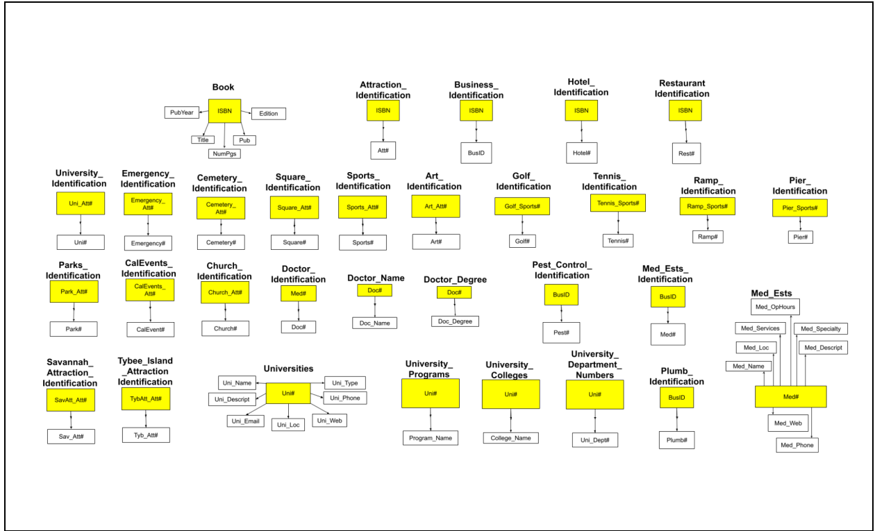
Figure 7: Diagram of the relations in 4NF
