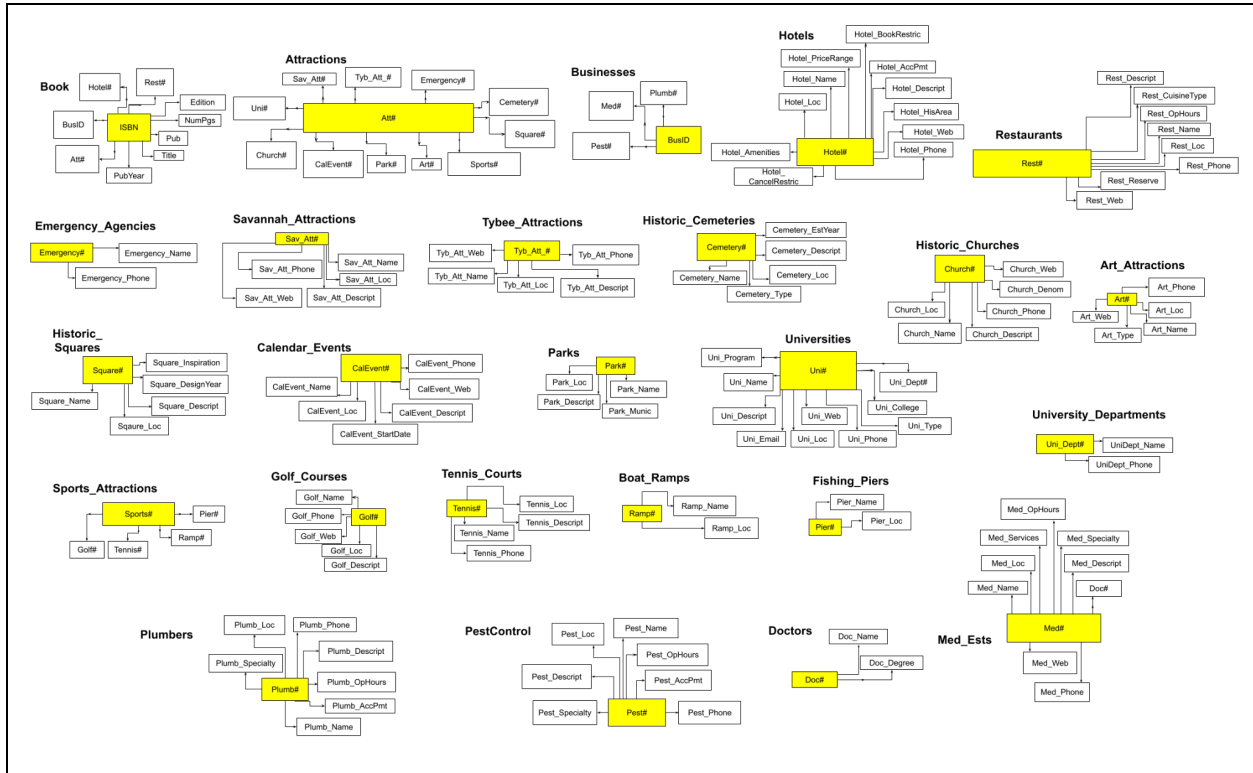
Figure 6: Diagram of the relations in BCNF (same as Figure 5)
