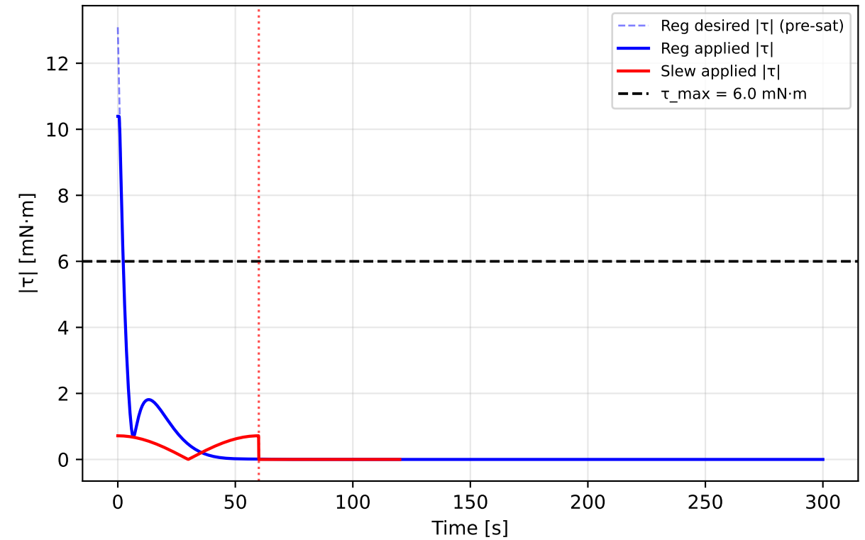
Near-IC (15°): regulator in linear regime, slew carries fixed overhead
