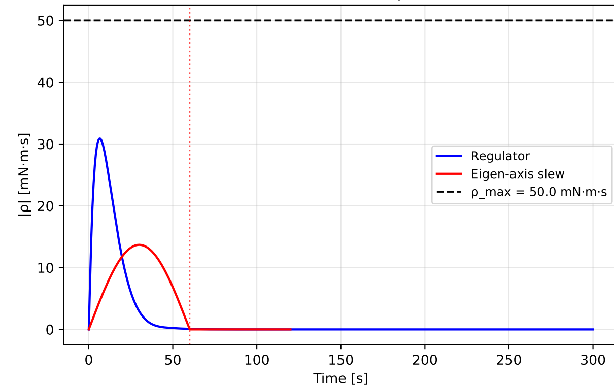
Wheel momentum buildup (150° IC)
