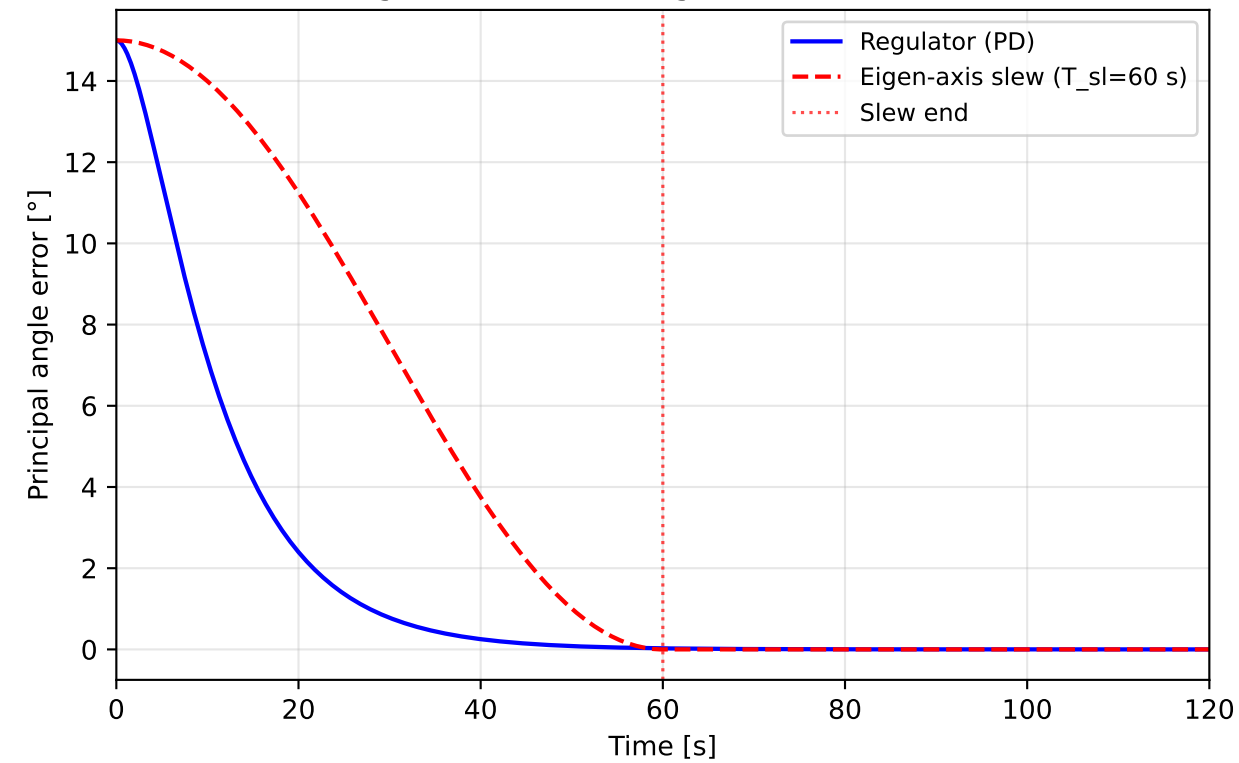
Near-IC (15°): regulator in linear regime, slew carries fixed overhead
