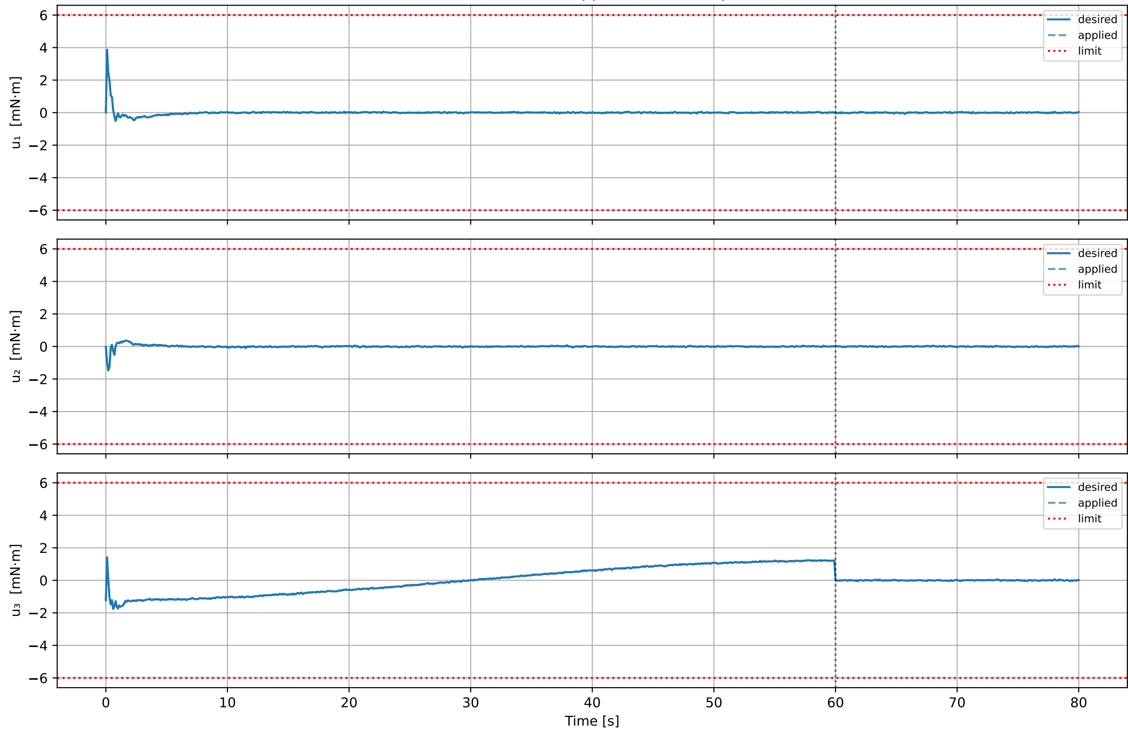
Commanded vs Applied Wheel Torque
