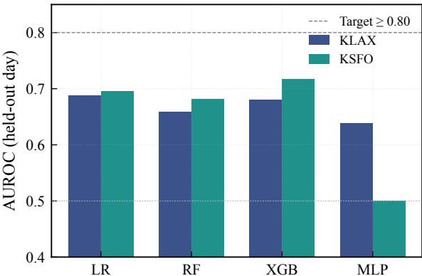
Risk-field AUROC (4-day train / 1-day test)
