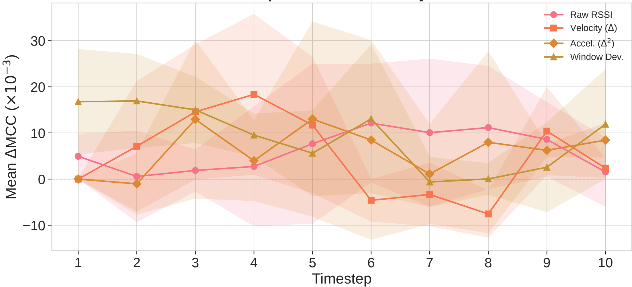
Feature Importance Over Time by Channel
