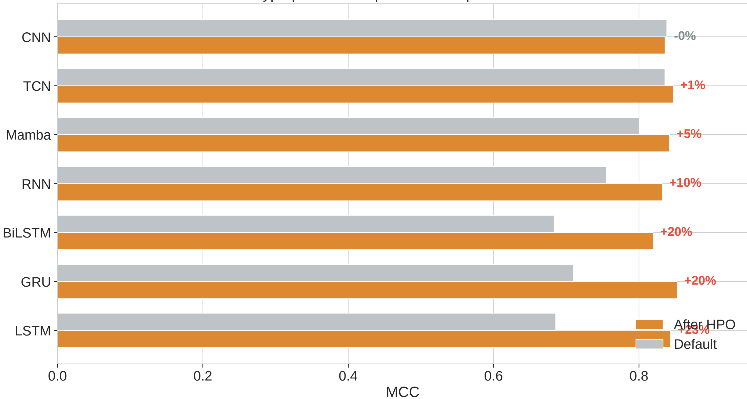
Hyperparameter Optimization Impact on MCC
