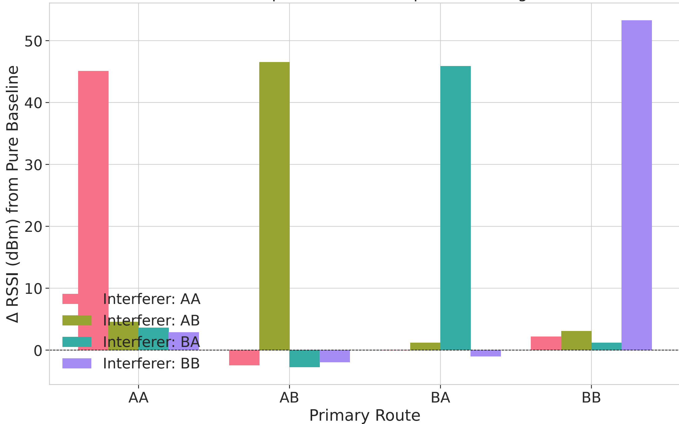
Interference Impact — RSSI Shift per Interfering Route
