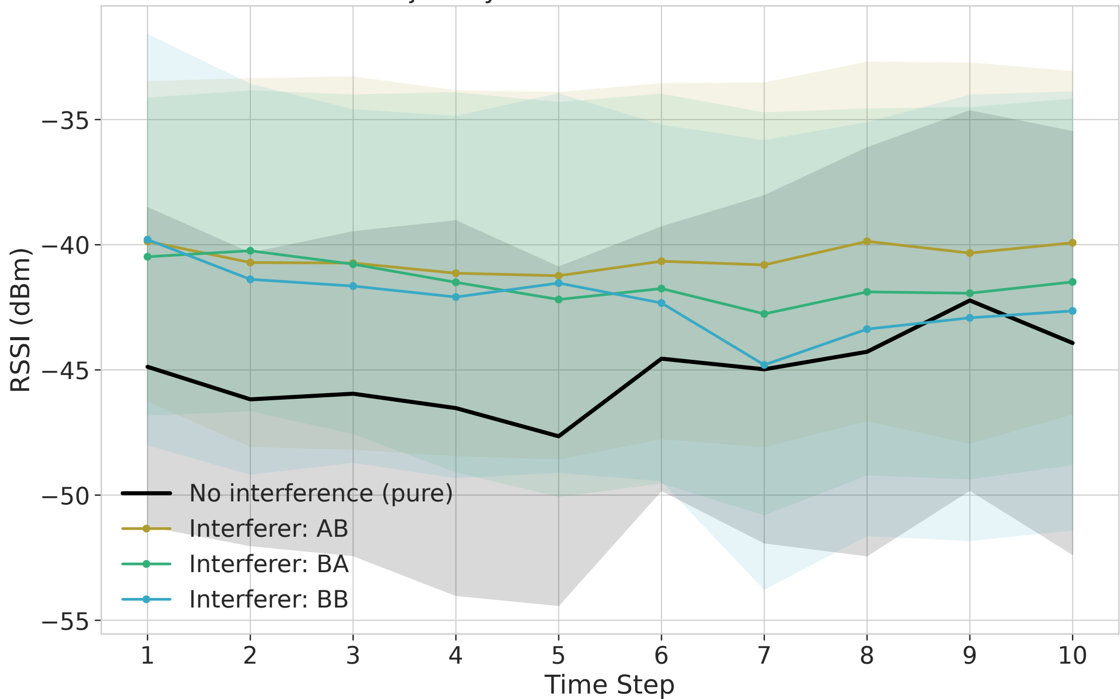
RSSI Trajectory — Route AA Under Interference
