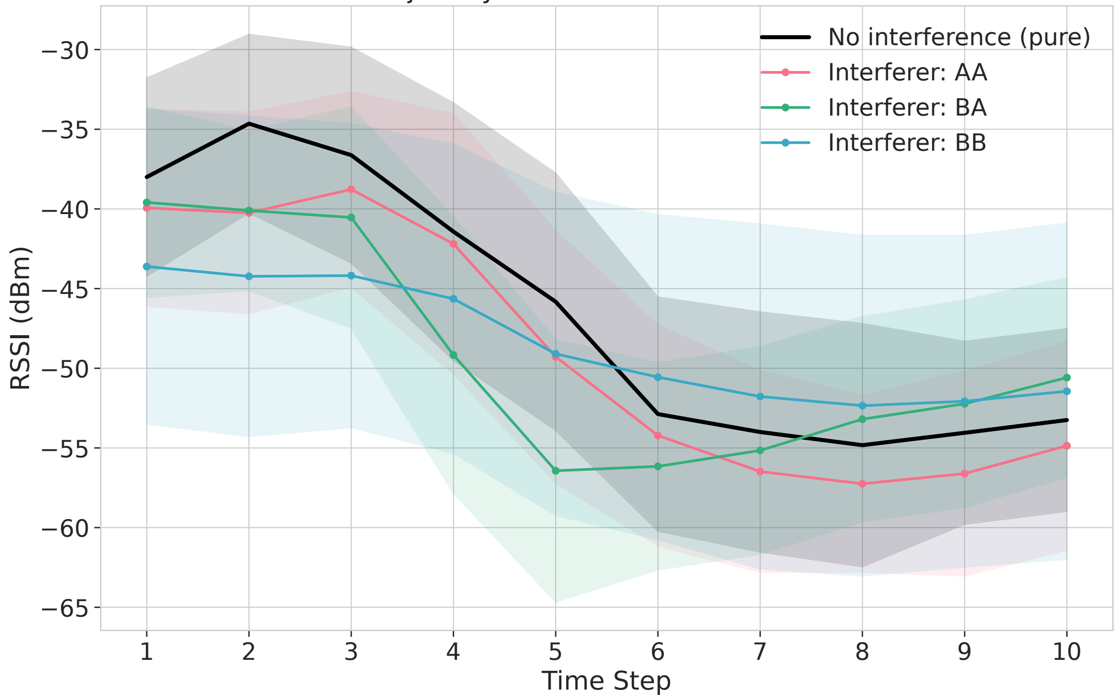
RSSI Trajectory — Route AB Under Interference
