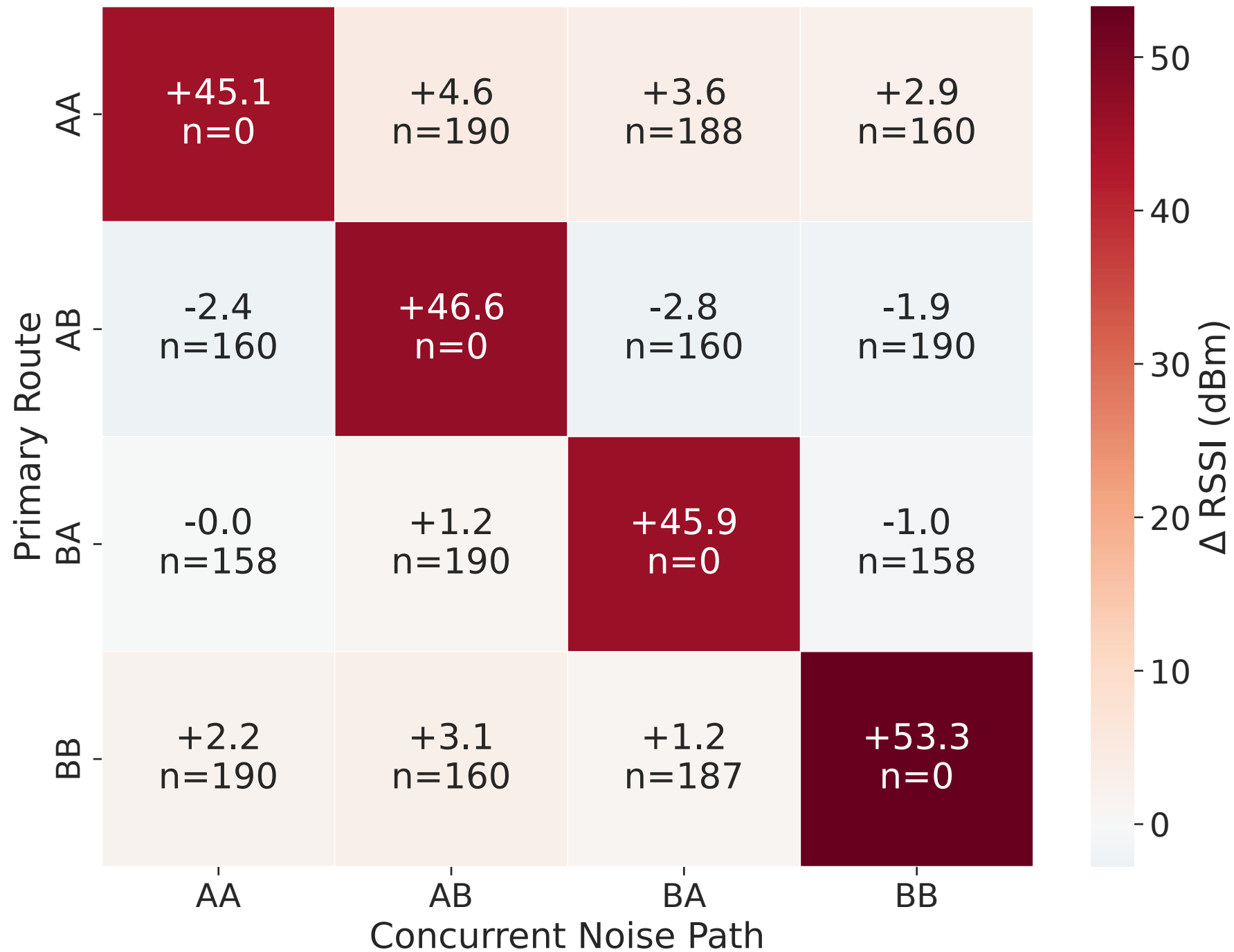
Interference Matrix — Mean RSSI Shift vs Pure Baseline
