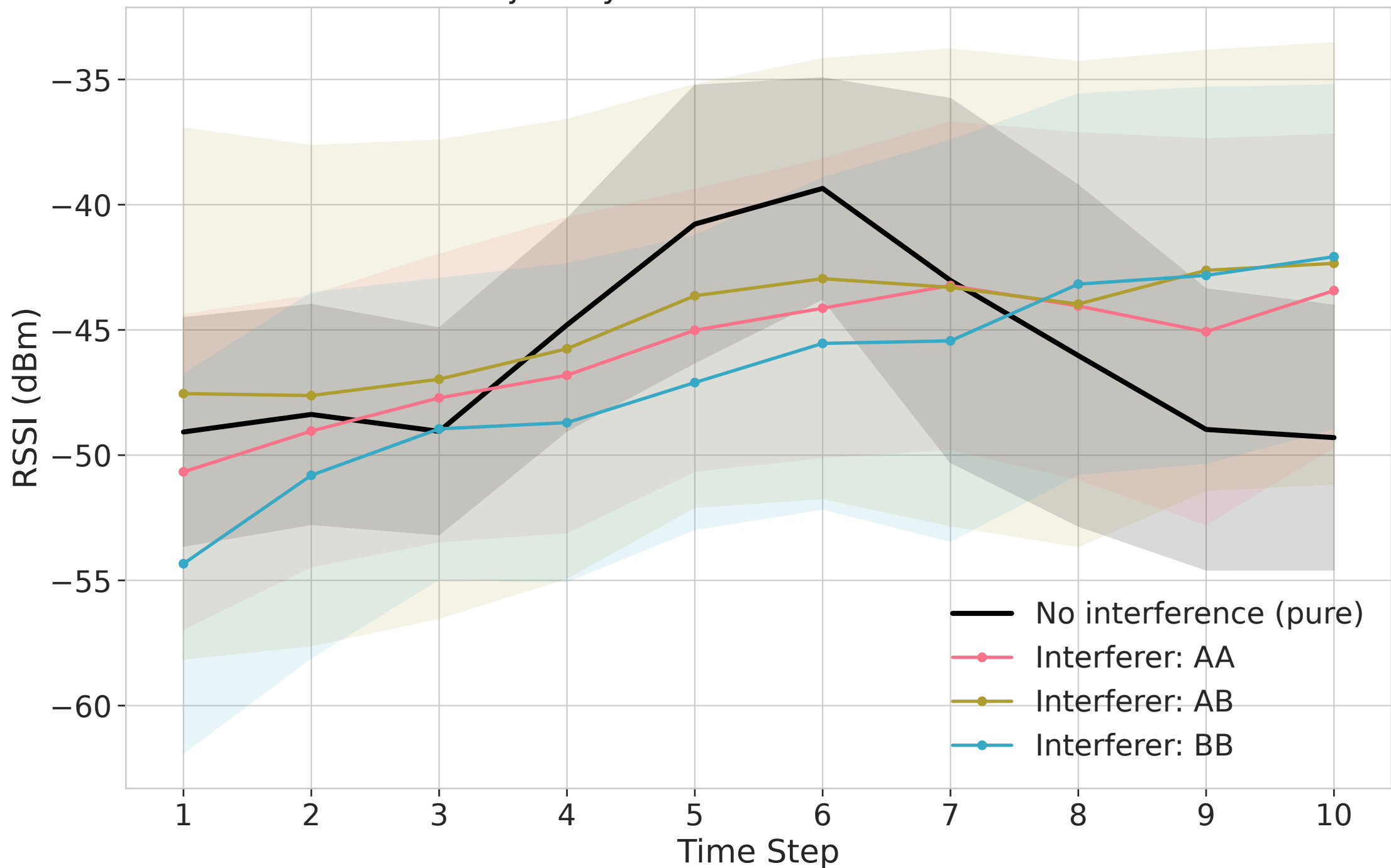
RSSI Trajectory — Route BA Under Interference
