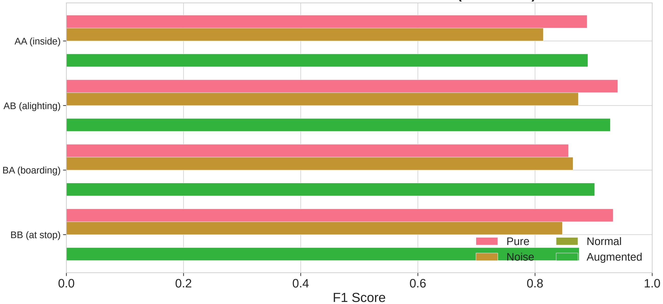
Per-Class F1 Score Across Dataset Variants (Best Model)
