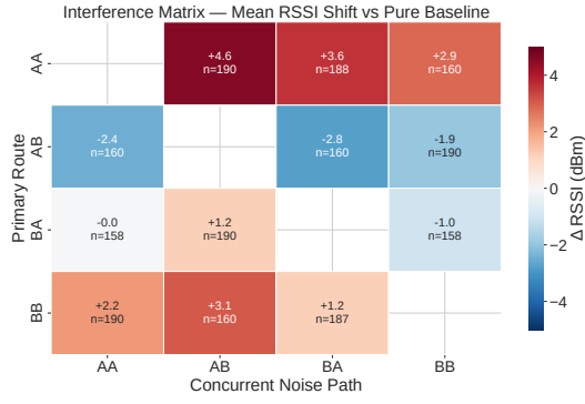
Figure 1. Interference heatmap: mean RSSI shift per (Route × Interferer) pair.
