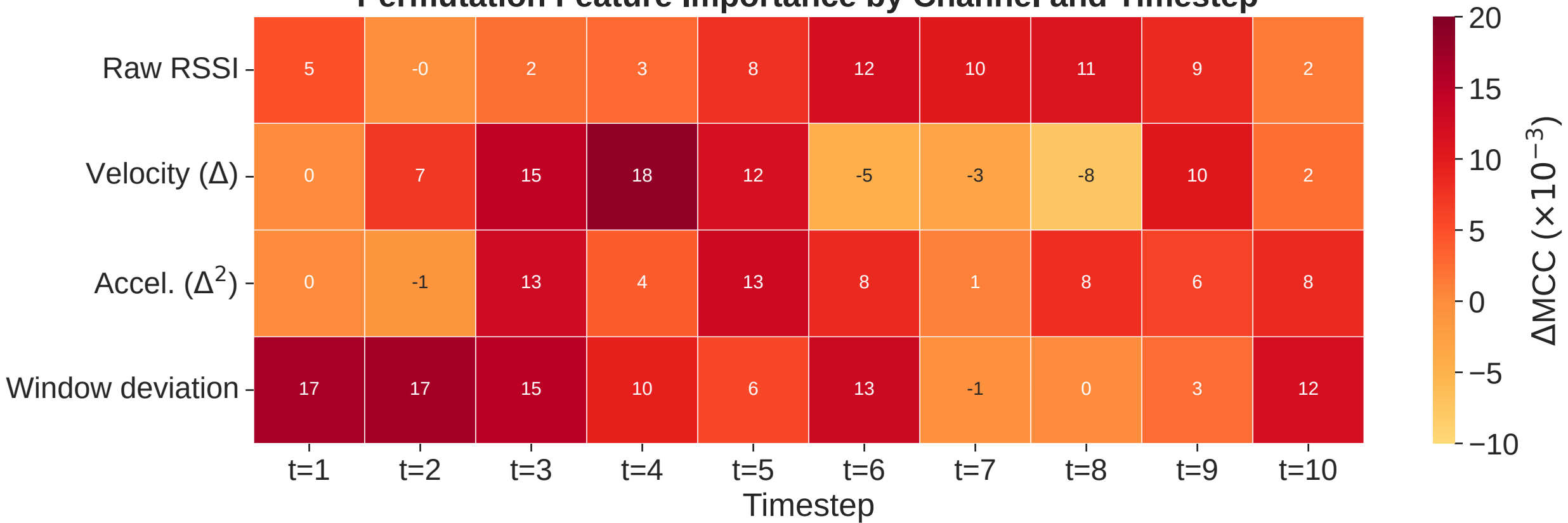
Permutation Feature Importance by Channel and Timestep
