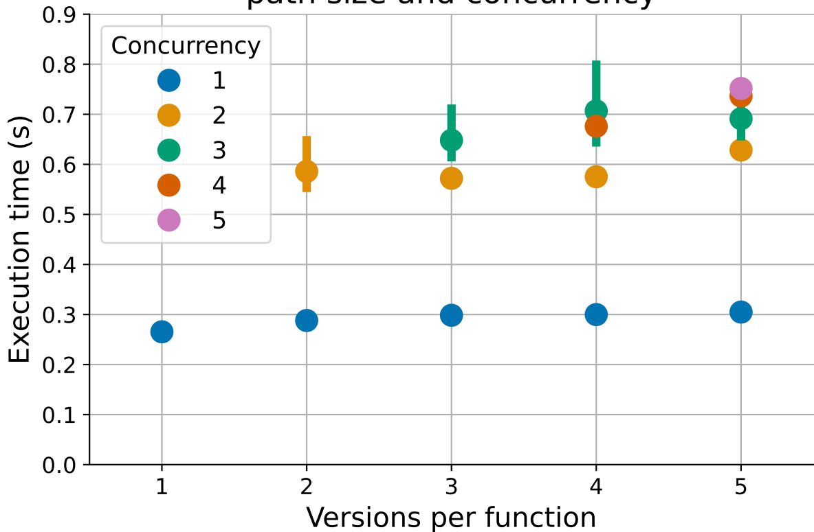
Execution time varying the path size and concurrency
