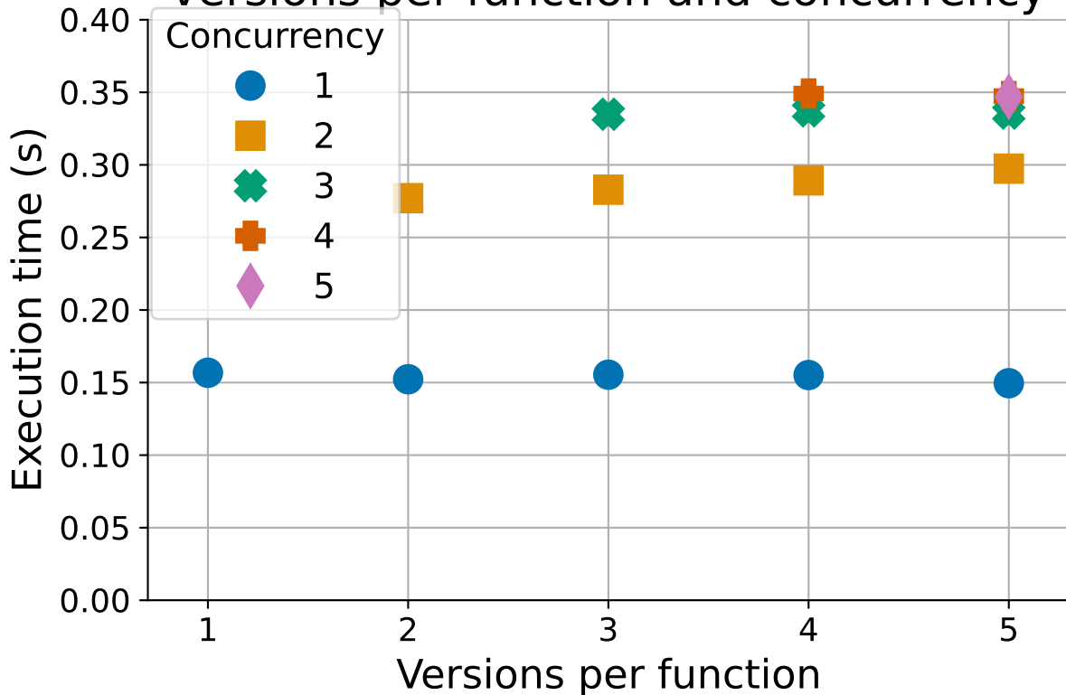
Execution time varying the number of versions per function and concurrency
