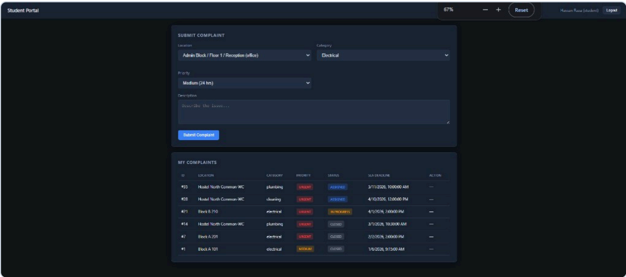
Figure 2 — Student Portal
