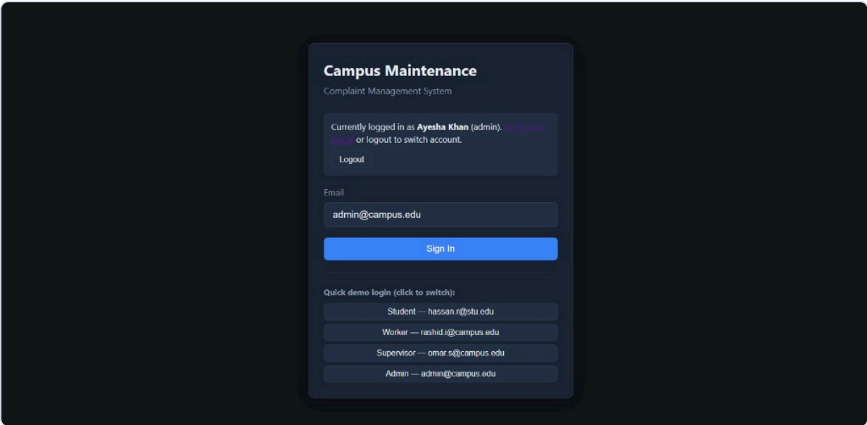
Figure 1 — Login Page
