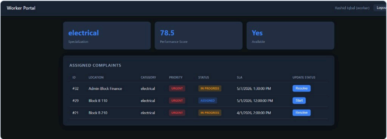
Figure 3 — Worker Portal
