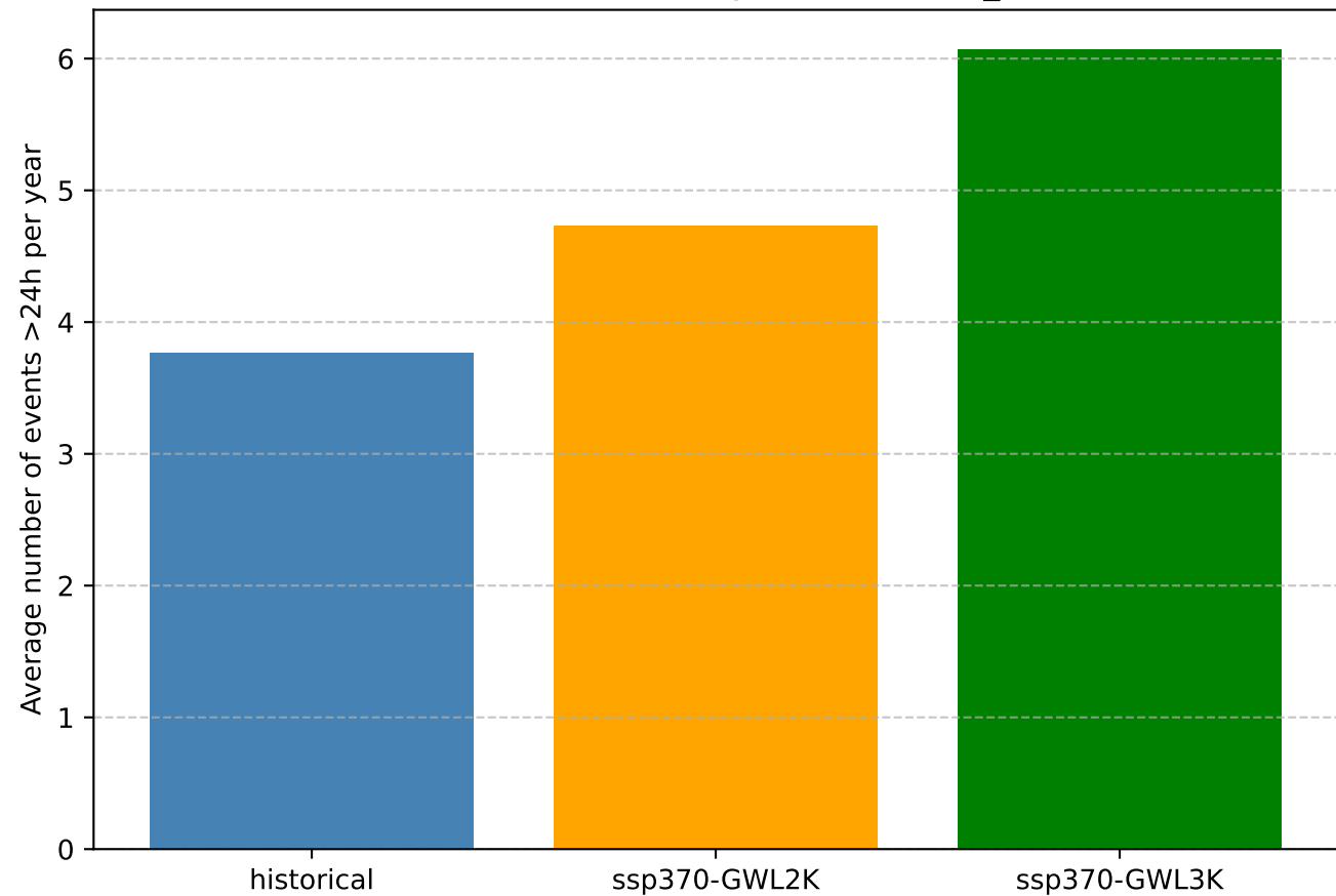
Dunkelflaute events longer than 24h (3_3MW)
