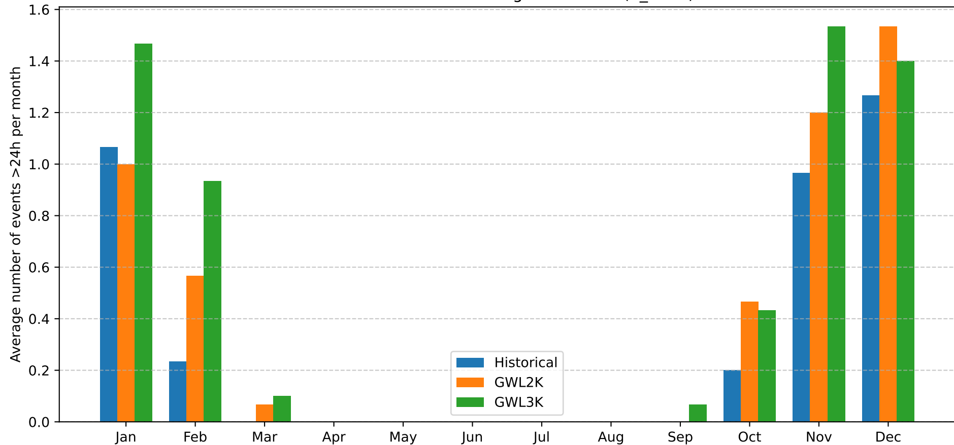
Dunkelflaute events longer than 24h (3_3MW)
