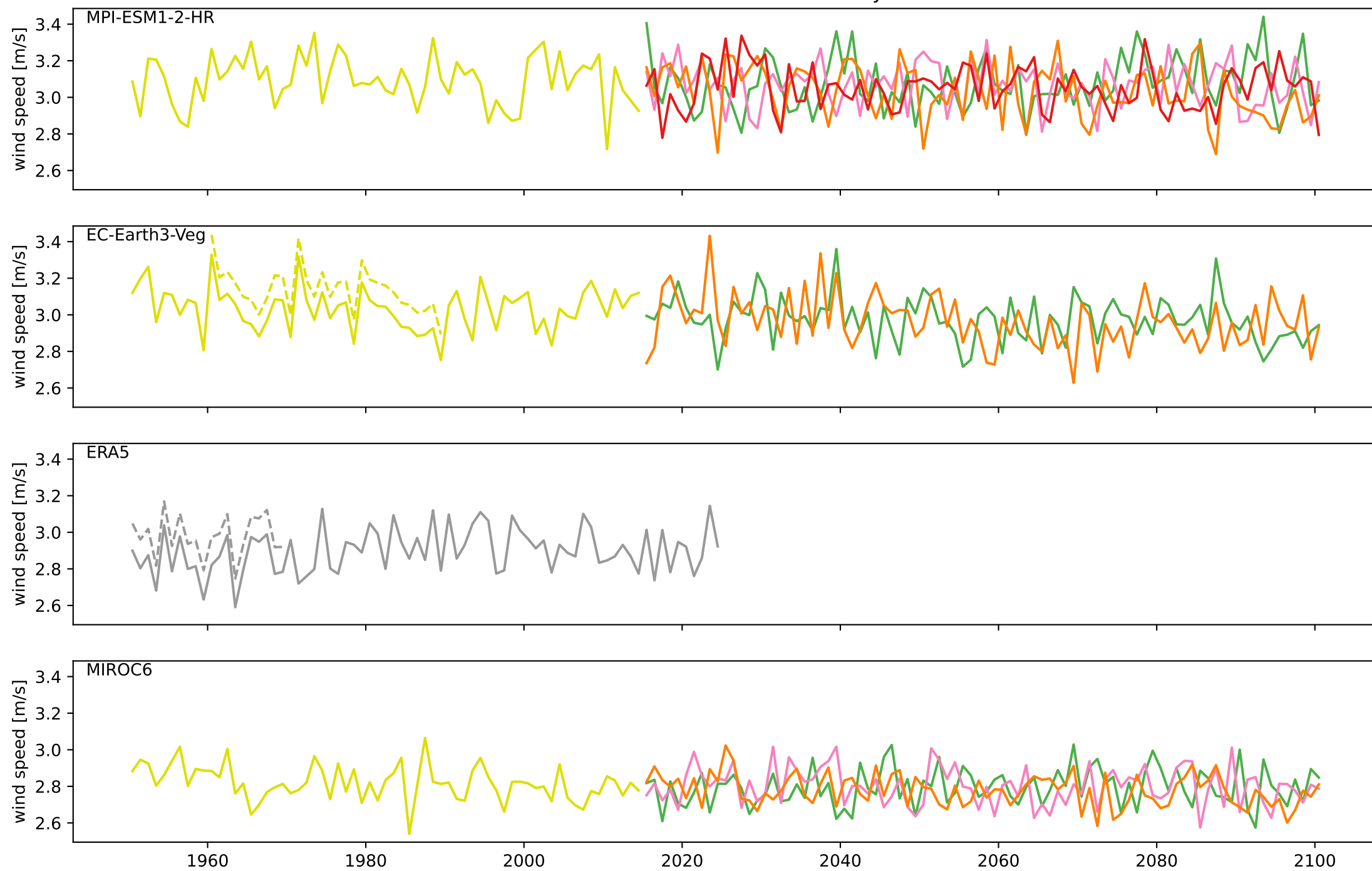
Annual mean sfcWind Germany
