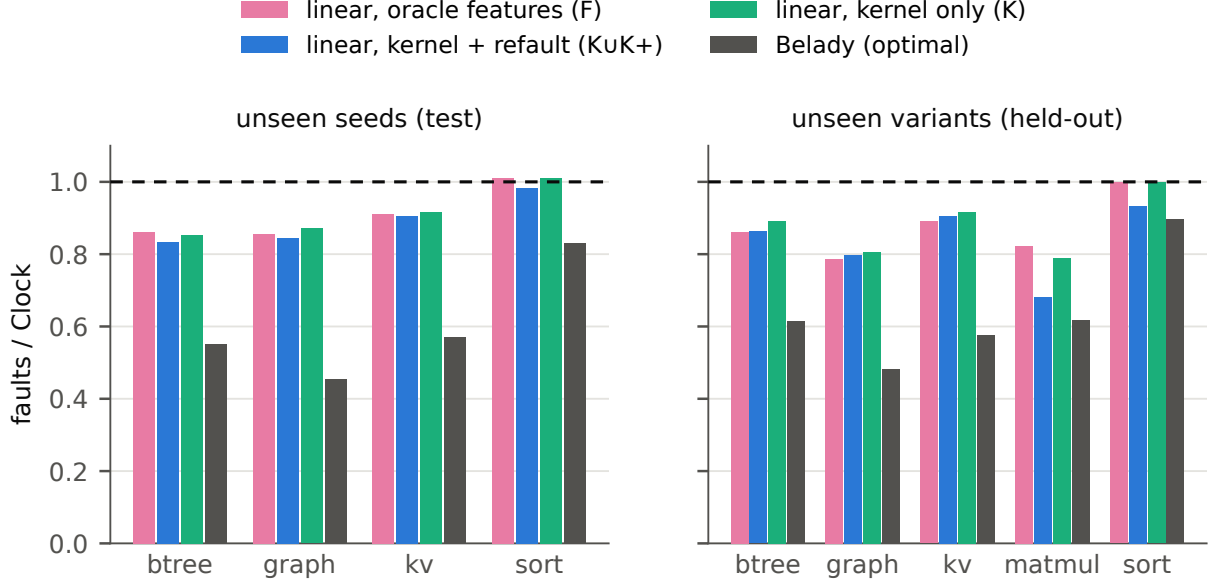
Figure 4: The best linear model of each feature tier, chosen on validation, relative to Clock (averaged over 5/10/20% memory). Lower is better.
