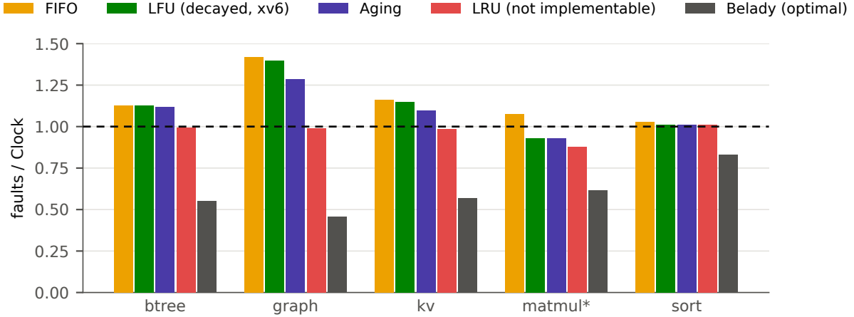
Figure 2: The policies a kernel has today. Each bar is a policy’s faults divided by Clock’s on the same traces (test traces, *matmul: held-out; averaged over 5/10/20% memory). The dashed line is Clock: above it is worse, below it is better. The dark bar is Belady, the best possible, so the gap between the line and the dark bar is the room for a better policy.
