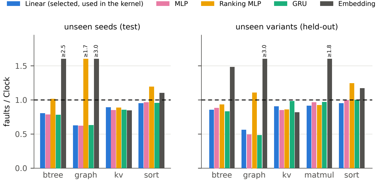
Figure 5: The five model types compared: faults relative to Clock (dashed line), each benchmark’s own model, 10% memory. Bars that would go off the chart are cut at 1.6 and labelled with their value ( \geq : the run was stopped once it reached that many times Clock’s faults).
