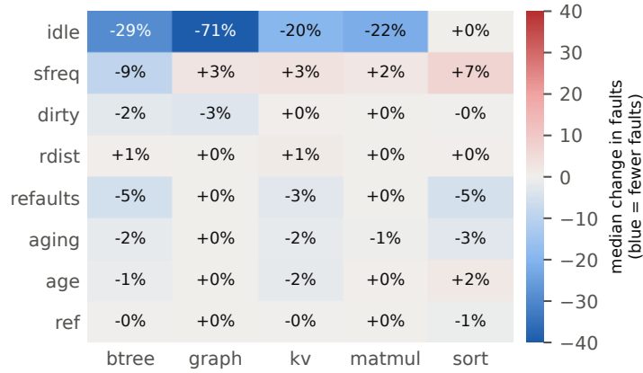
Figure 3: What each kernel feature adds: the median change in faults when the feature is added to a feature set that does not have it, over all such pairs of sets (per-workload models; test, matmul held-out).
