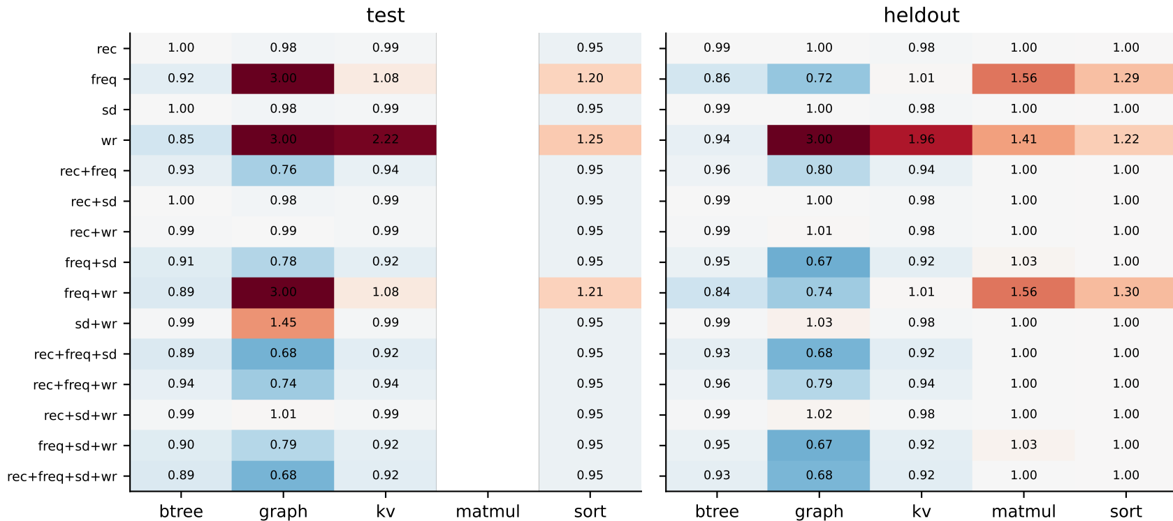
All 15 full-stream feature subsets, linear, global model (faults / Clock; blue = better)
