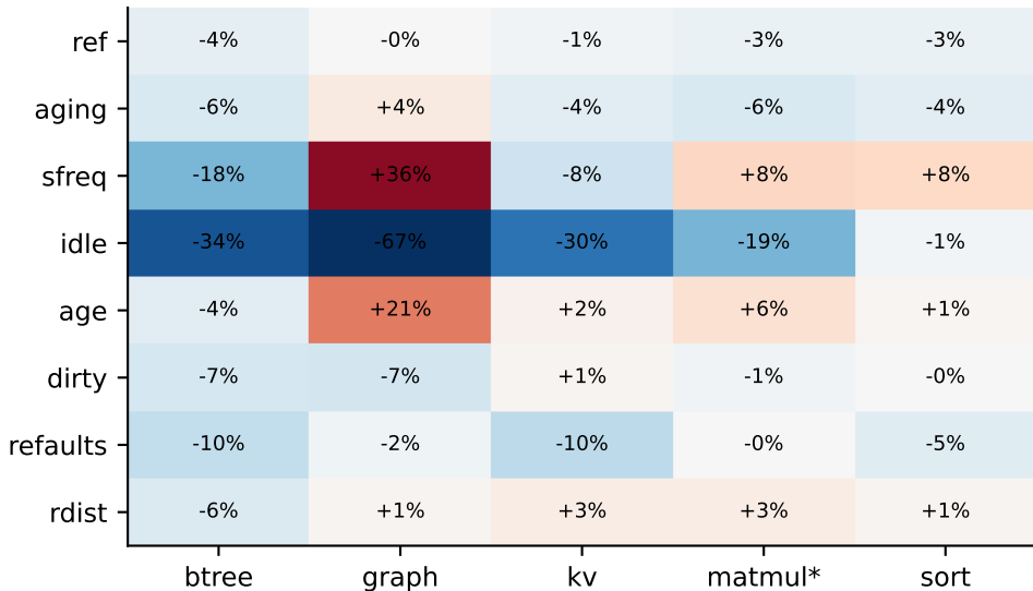
Average change in faults from adding a feature (over all kernel subsets lacking it; test, *held-out; blue = helps)
