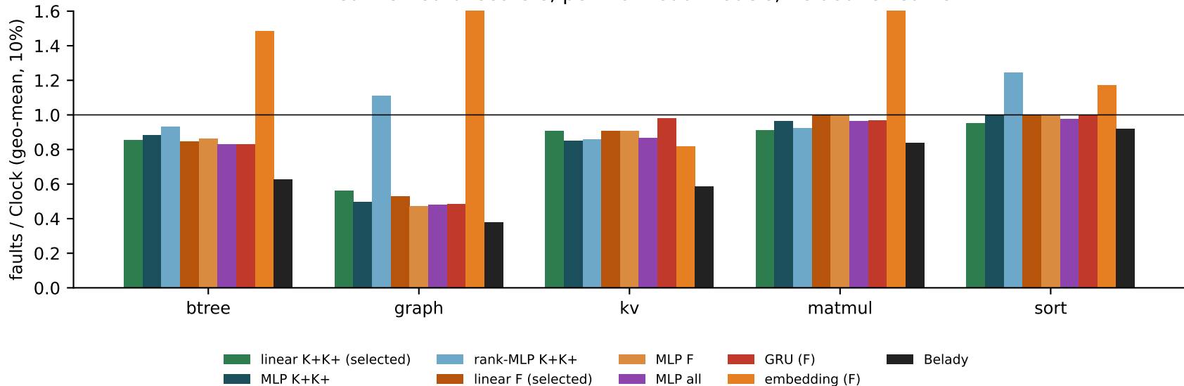
Linear vs neural scorers, per-workload models, heldout streams
