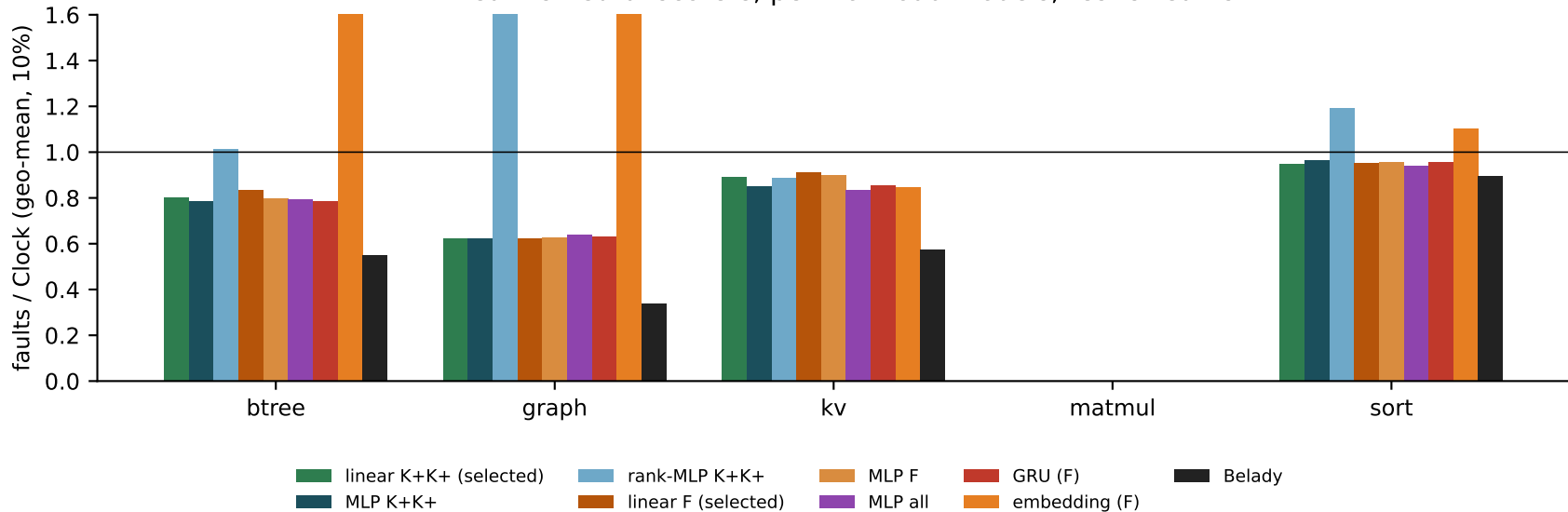
Linear vs neural scorers, per-workload models, test streams
