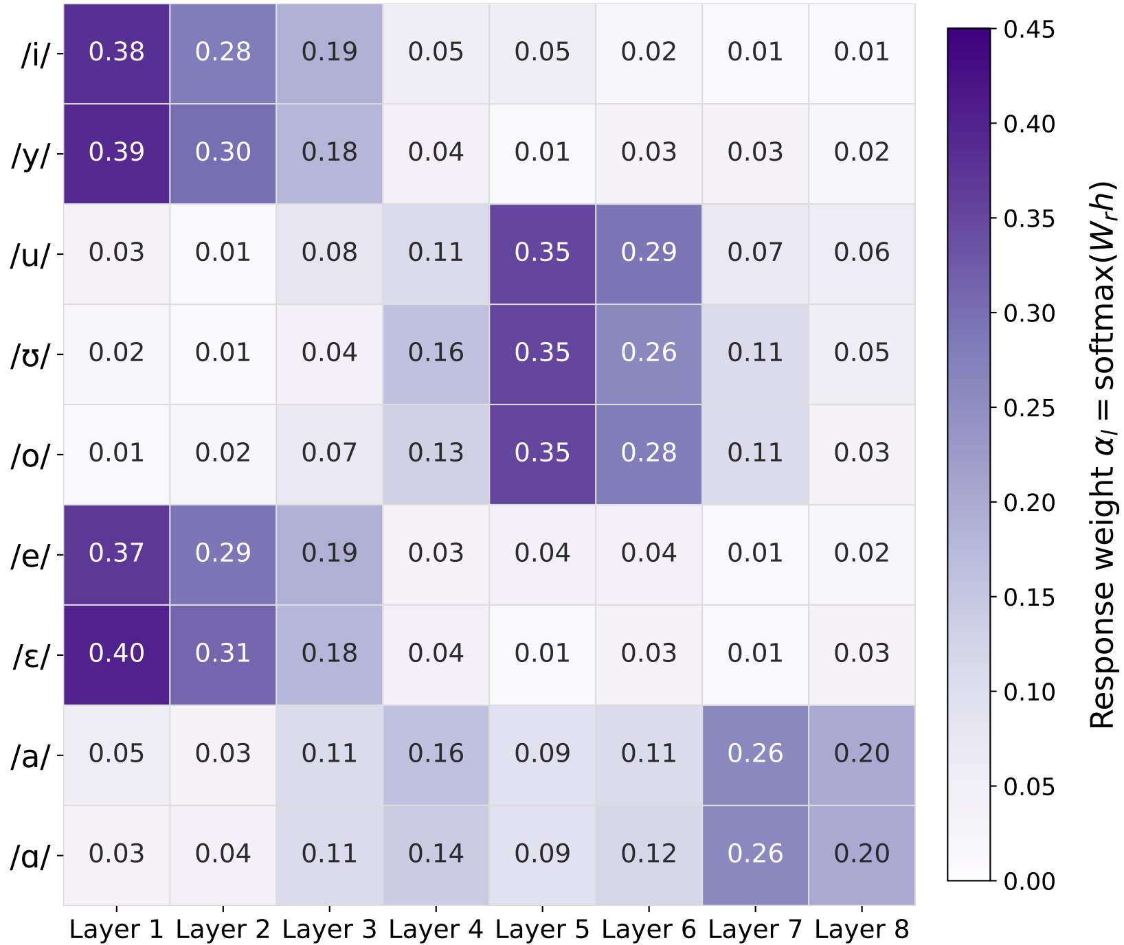
Layer-wise Prompt Projections
