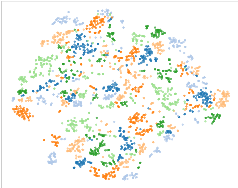
Downstream t-SNE colored by regions (b) RPL Only Silhouette = 0.04
