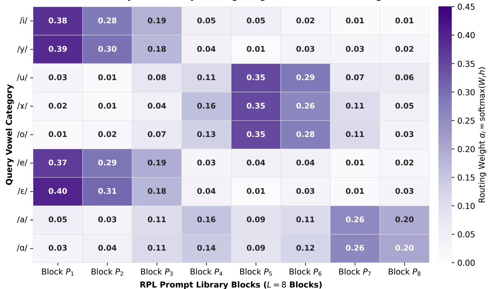
RPL Internal Dynamic Query Routing Weights across Vowel Categories
