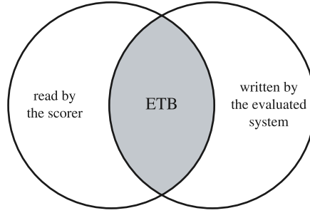
Figure 1: The left set holds the rubric, frozen ground truth, and the judge’s own structured output. The right holds the answer, its reasoning, tool arguments, stdout, and the transcript. The invariant says the overlap must be empty; each class in Table 1 is one way it stopped being.
