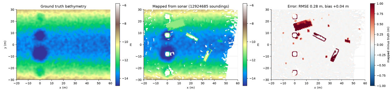
Figure 12: Ground truth bathymetry, the map built from simulated sonar during the mission, and the difference. The residual is near zero over open bed; the remaining structure is the submerged objects, which stand above the bare bed and are the subject of Section 7.
