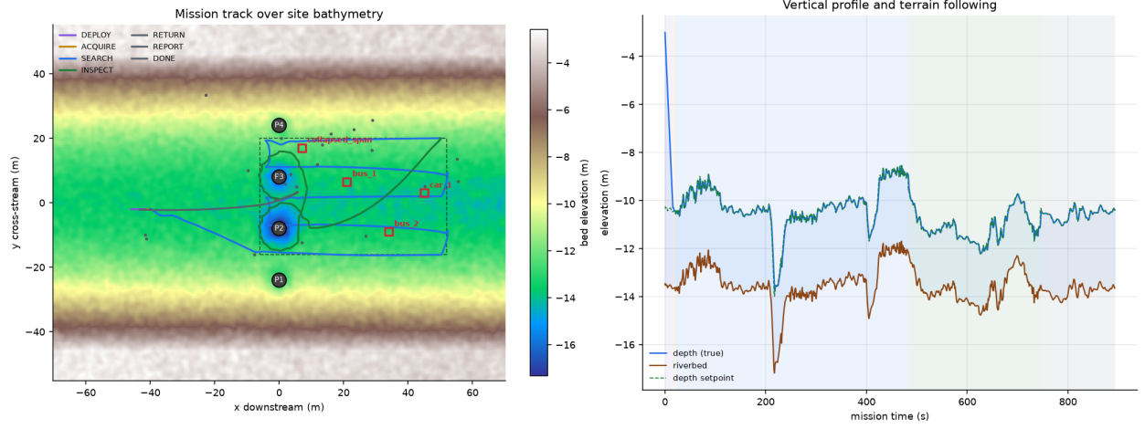
Figure 10: Mission track over site bathymetry, coloured by mission phase, and the vertical profile showing terrain following against the riverbed.
