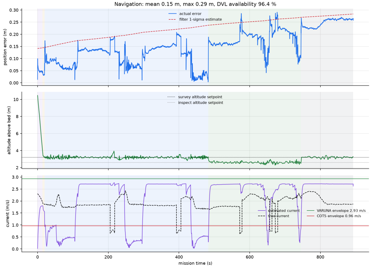
Figure 11: Navigation error against the filter's own uncertainty estimate, altitude tracking, and estimated against true current with both vehicle envelopes marked.
