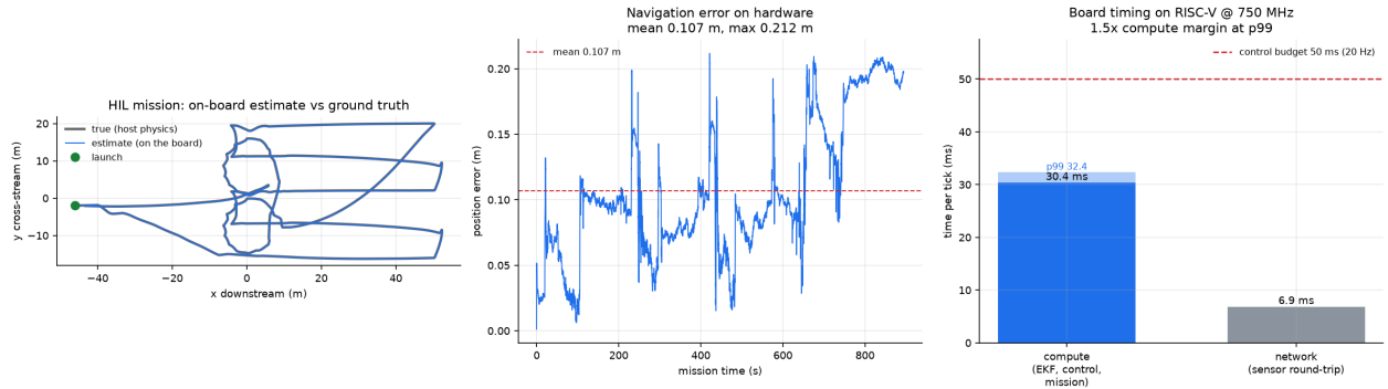
Figure 16: Full mission executed on the flight computer. Left: the on-board pose estimate against the host’s ground truth. Centre: navigation error over the run. Right: per-tick board timing, compute separated from the sensor round-trip, against the control budget.
