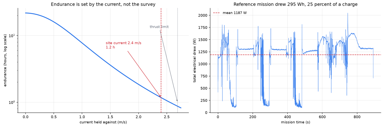
Figure 15: Left: endurance holding station, against the current being fought. Right: the electrical draw of the reference mission, integrated from the logged thruster forces. The low sections are downstream legs, the high ones are upstream legs and station keeping.
