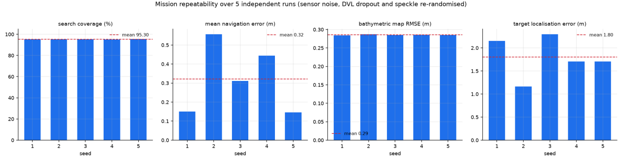
Figure 14: Per-seed results with the mean marked. The spread, not the best run, is the honest statement of what the system does.
