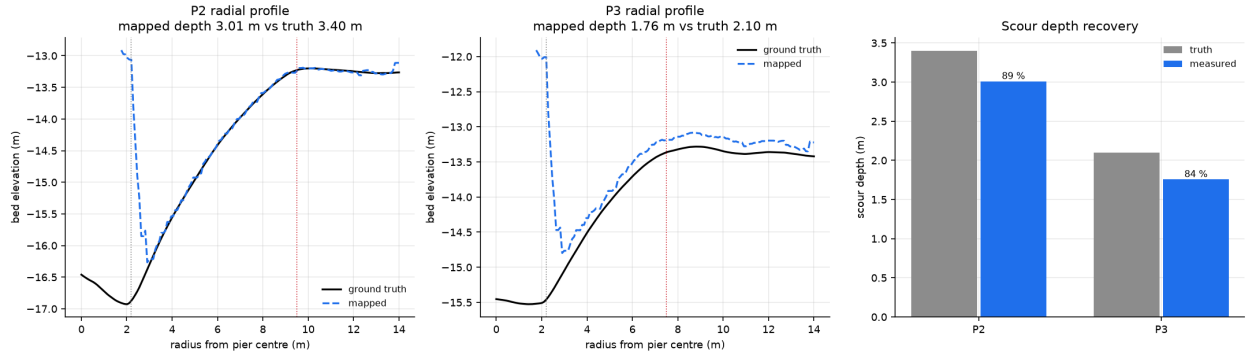
Figure 8: Radial bed profiles around the inspected piers, mapped against ground truth, and the resulting scour depth recovery.
